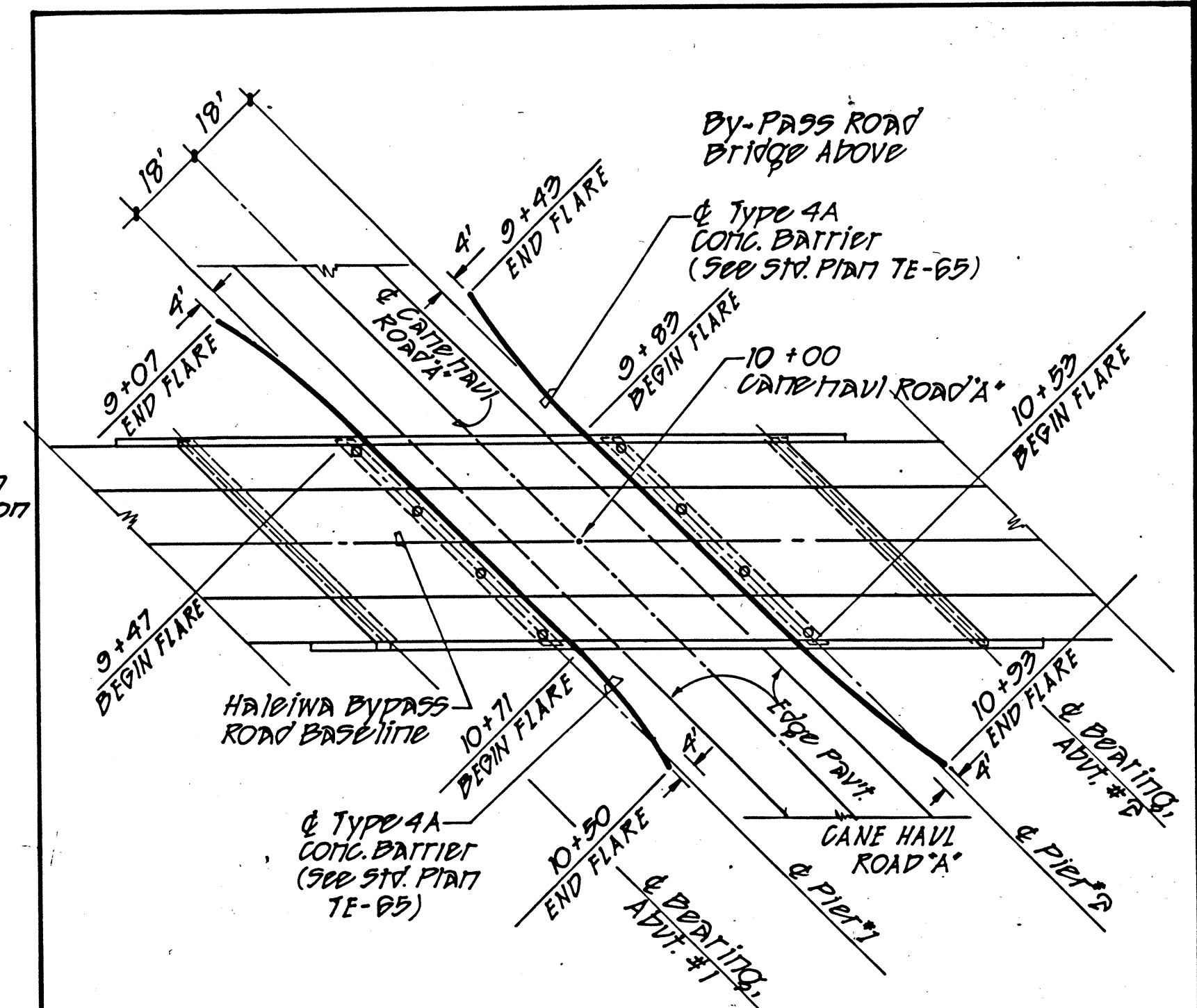
CANE HAVL ROAD BRIDGE CONCRETE BARRIER LAYOUT PLAN SCALE: 1" = 30'
