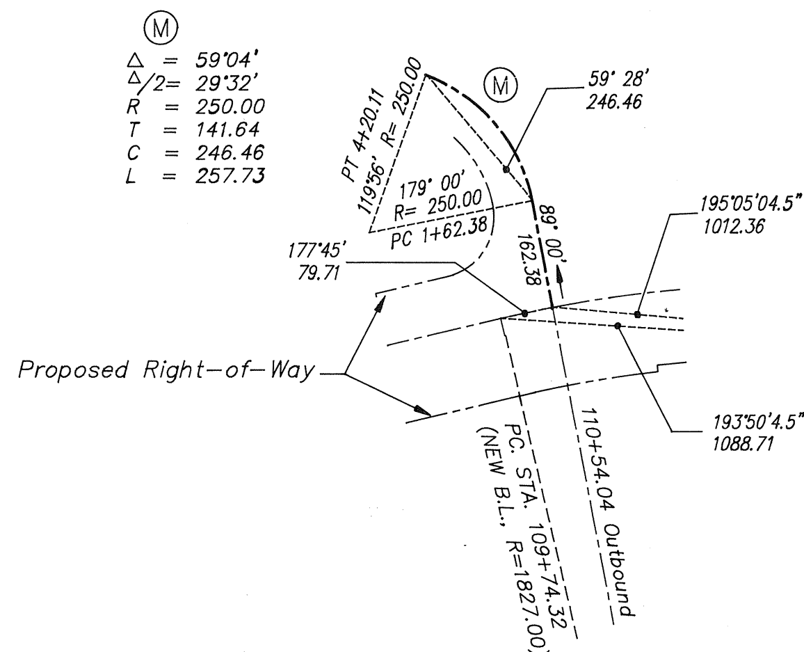
HALEIWA CONNECTOR INSET "C" Scale 1 in. = 200 ft.
