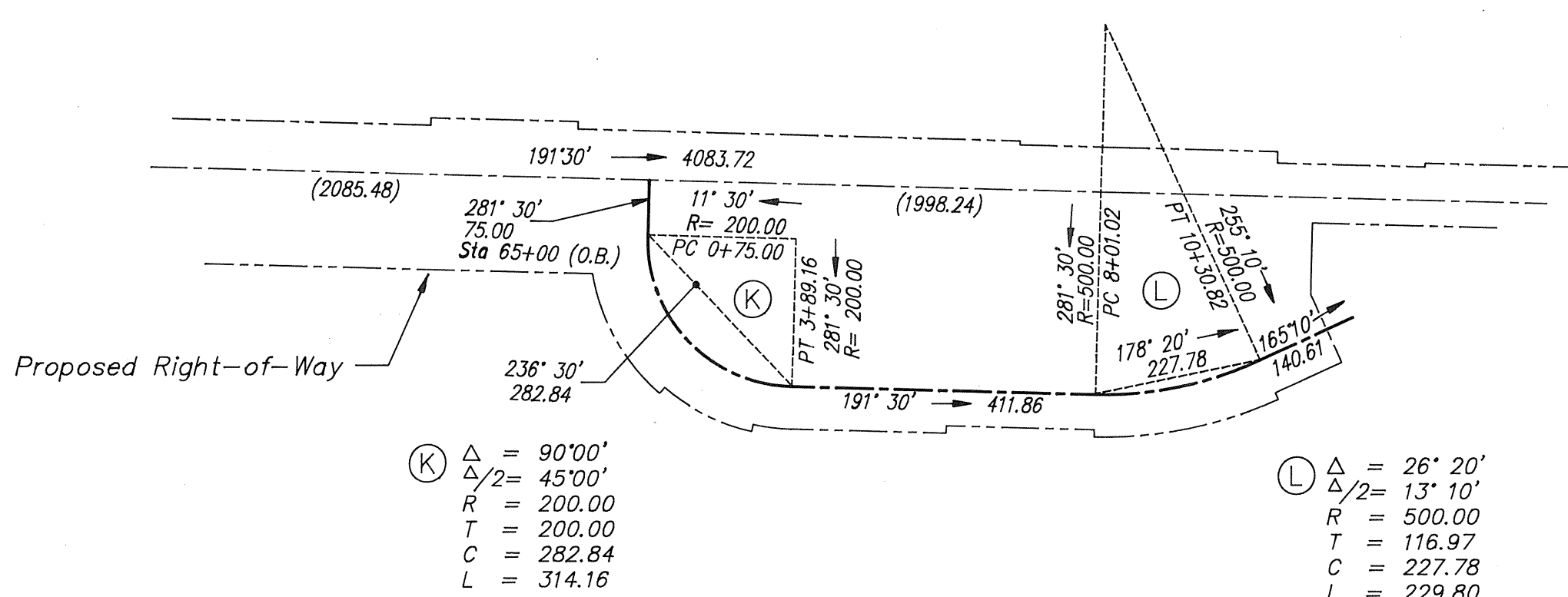
EMERSON ROAD INTERSECTION INSET "B" Scale 1 in. = 200 ft.
