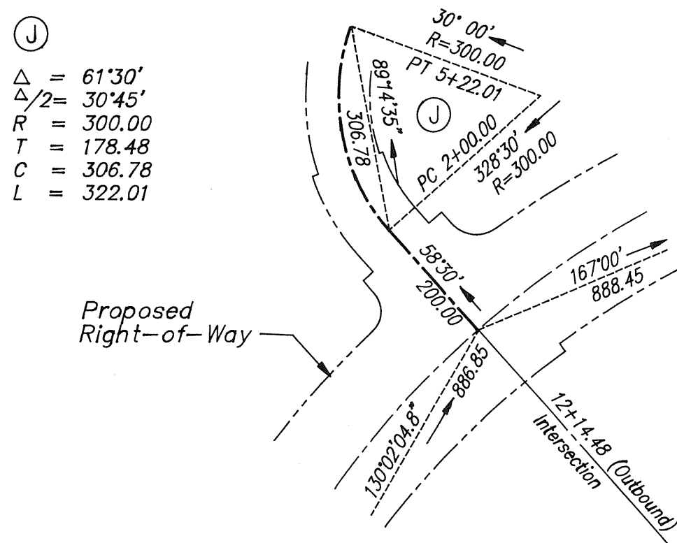
WAIALUA CONNECTOR INSET "A" Scale 1 in. = 200 ft.
