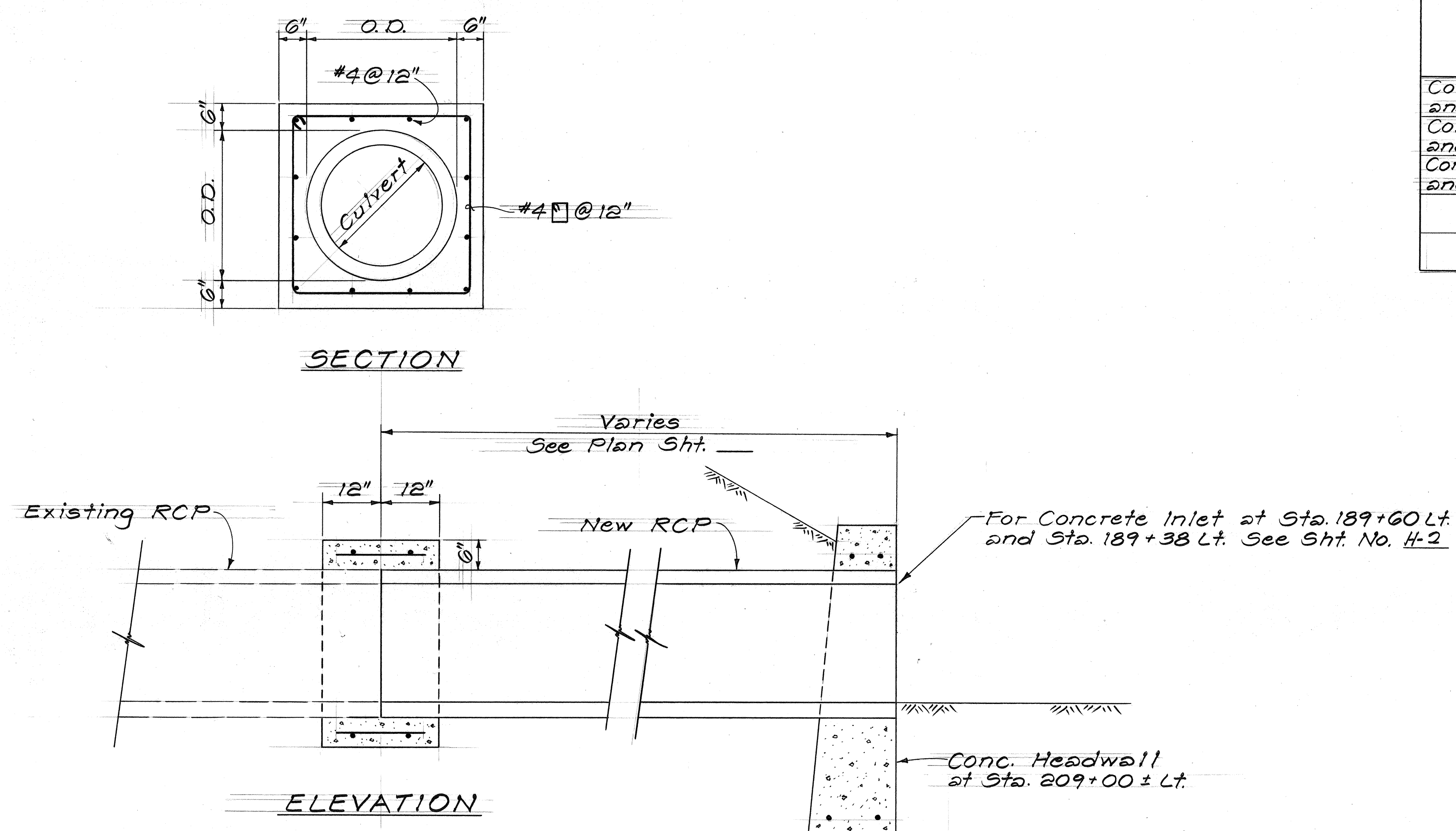
DETAIL OF CONCRETE COLLAR AND PIPE EXTENSION Scale: 3/4" = 1'-0"
