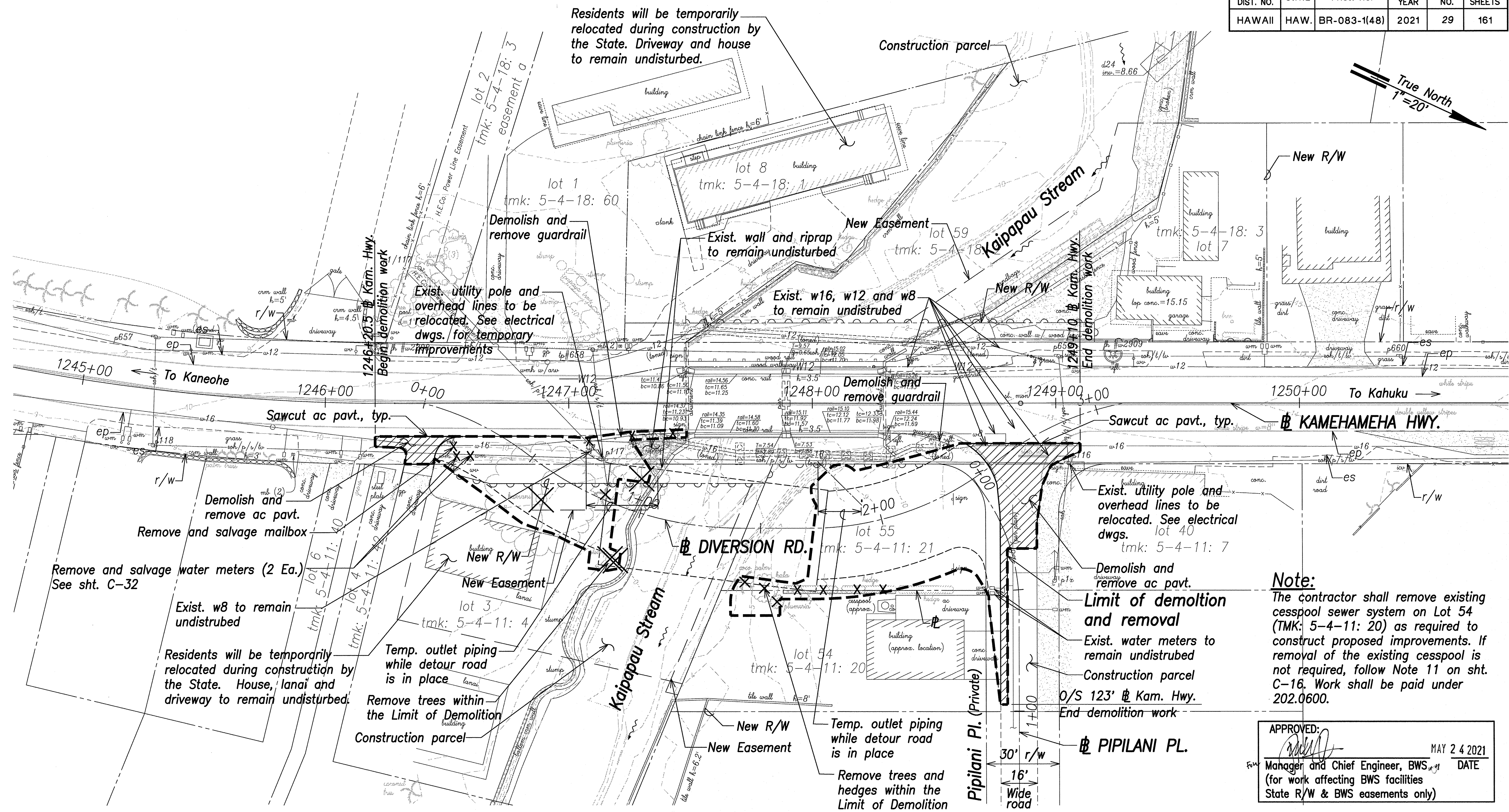
DIVERSION ROAD - EXISTING CONDITION & DEMOLITION PLAN Scale: 1"=20'
