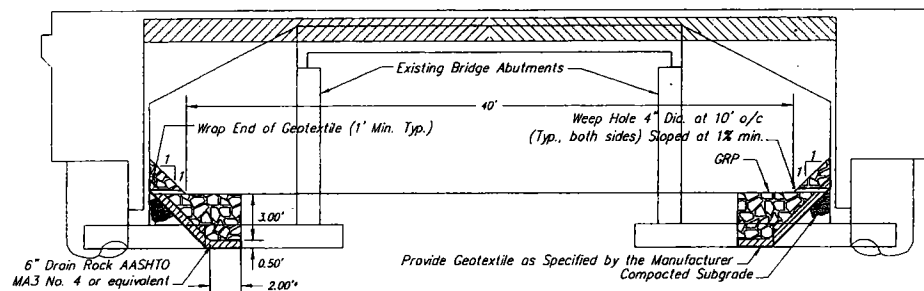
GRP Cross Section at Bridge Not to Scale
