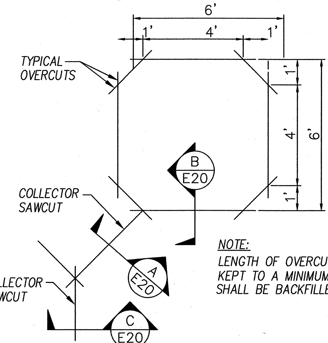
1 TYPICAL SENSOR LOOP SAWCUT DETAIL NOT TO SCALE
