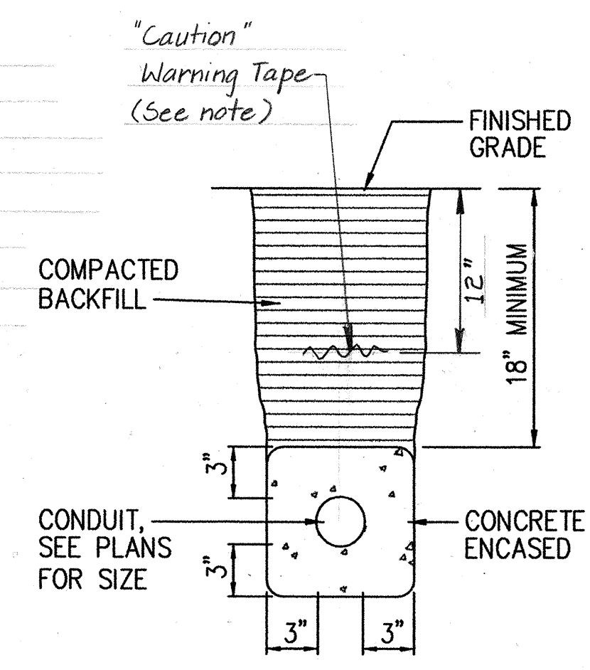
3 DUCT SECTION NOT TO SCALE
