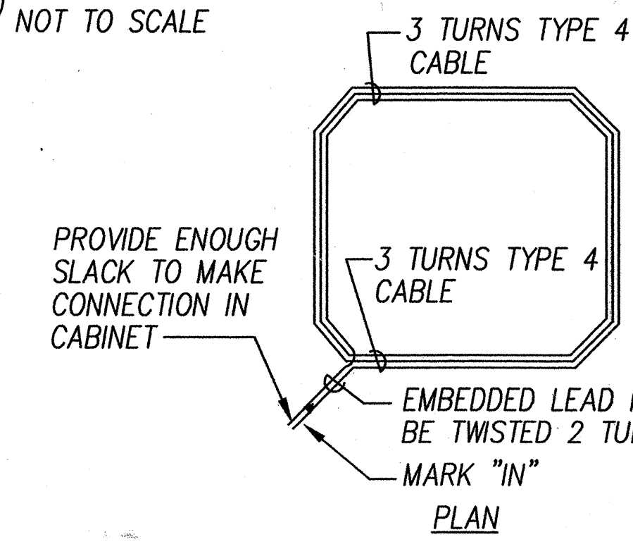
2 TYPICAL SENSOR LOOP WIRING DIAGRAM NOT TO SCALE
