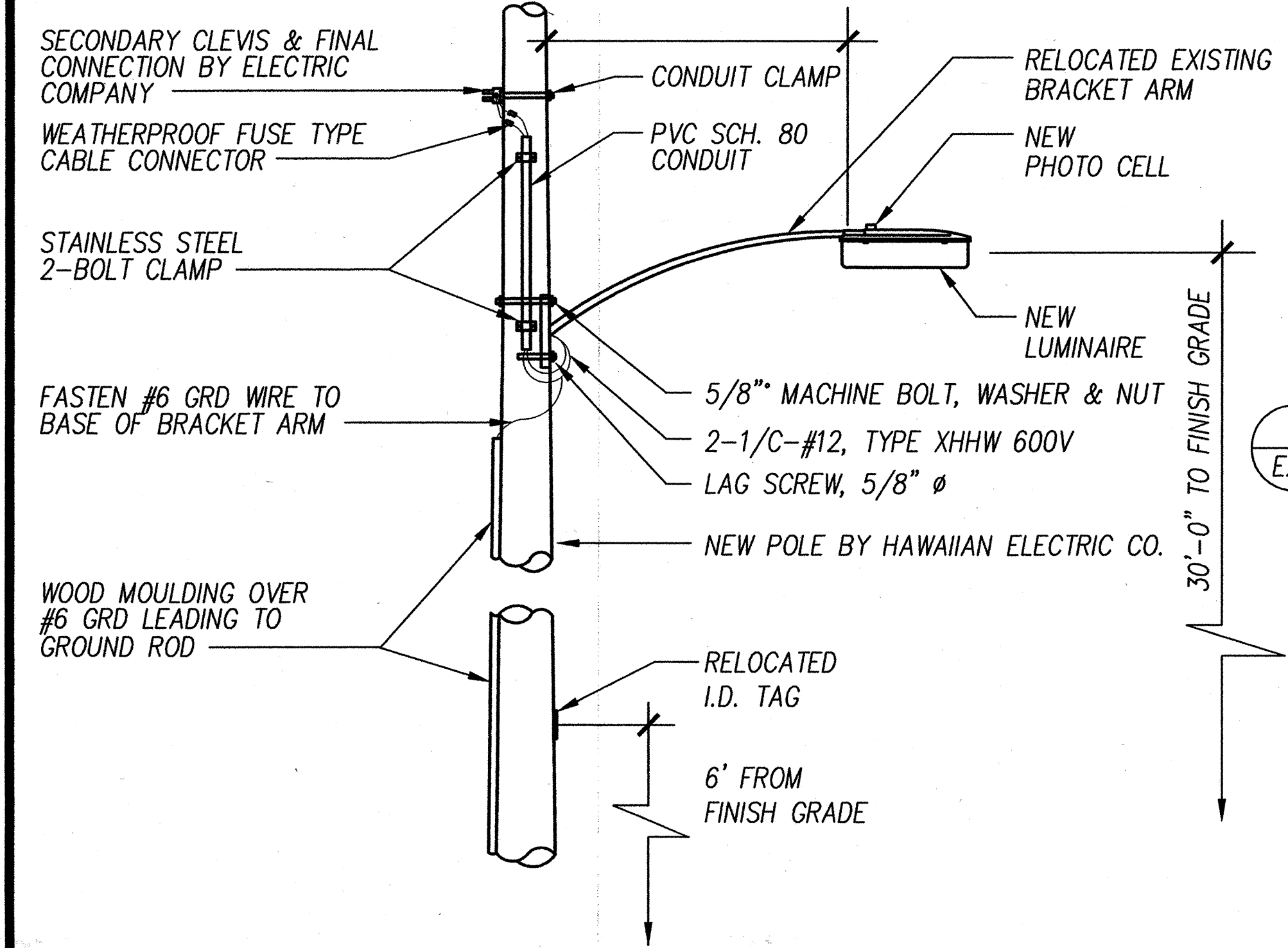
WOOD POLE STREET LIGHT MOUNTING DETAIL NOT TO SCALE
