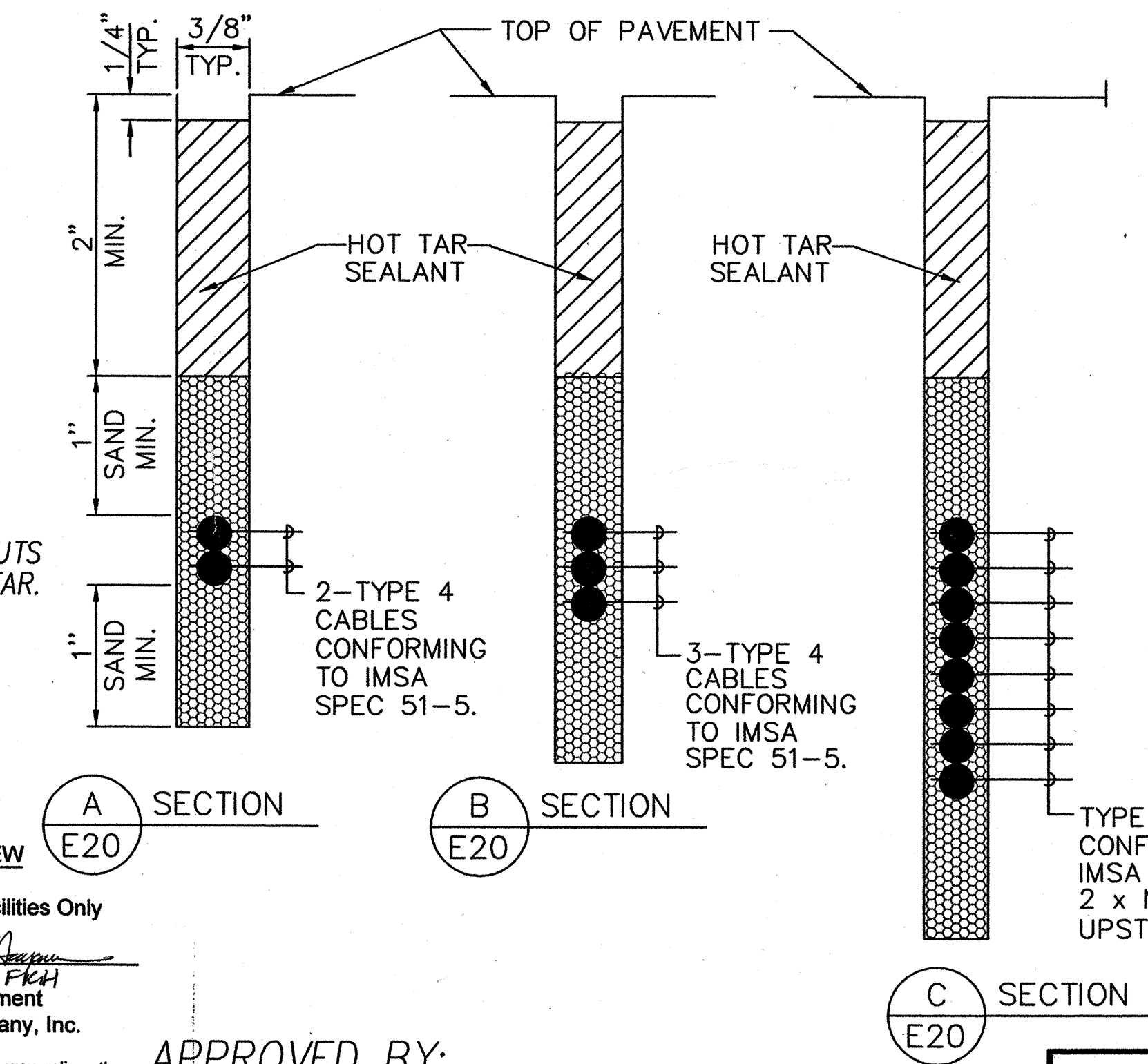
1 TYPICAL SENSOR LOOP SAWCUT DETAIL NOT TO SCALE
