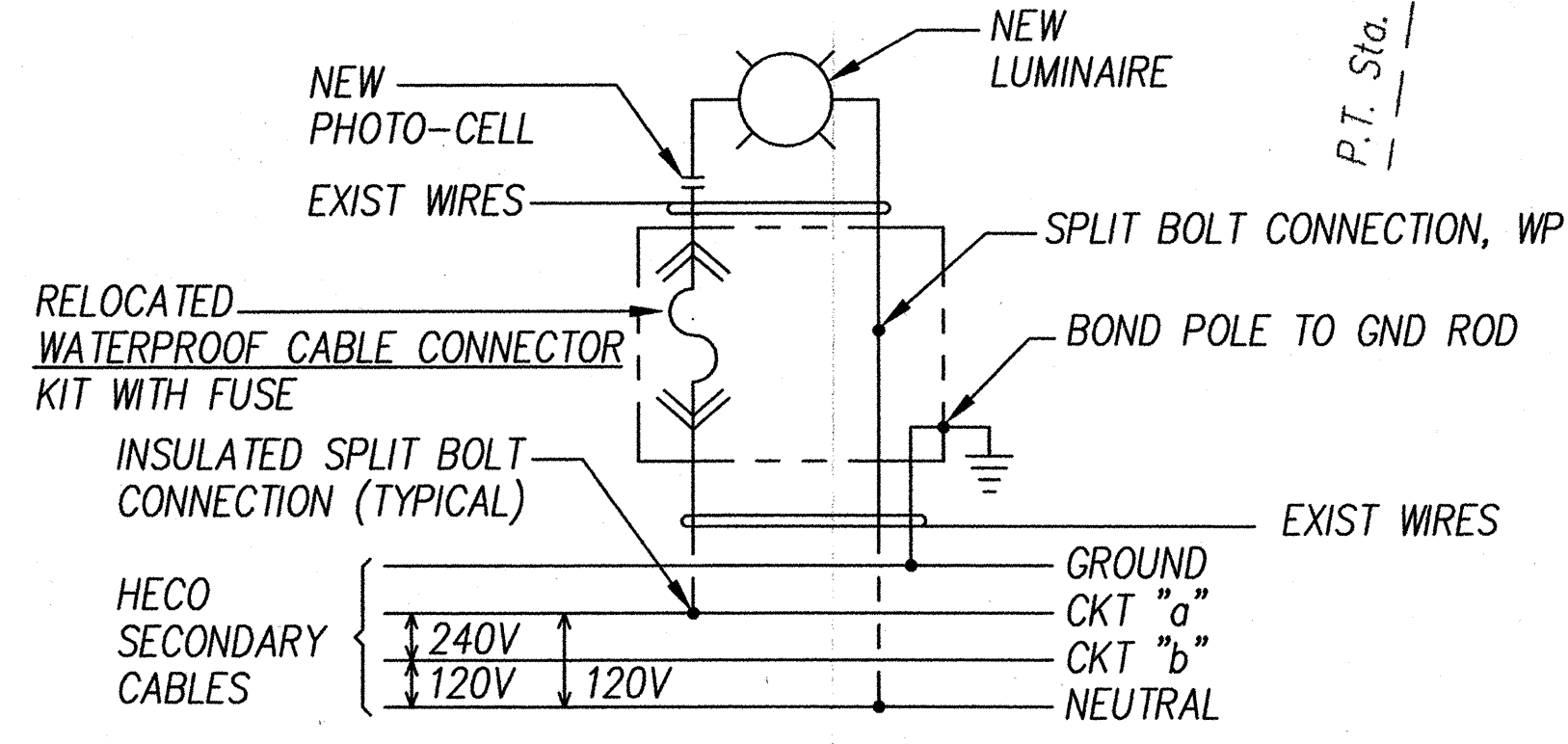
TYP. HIGHWAY LUMINAIRE CONNECTION DIAGRAM NOT TO SCALE
