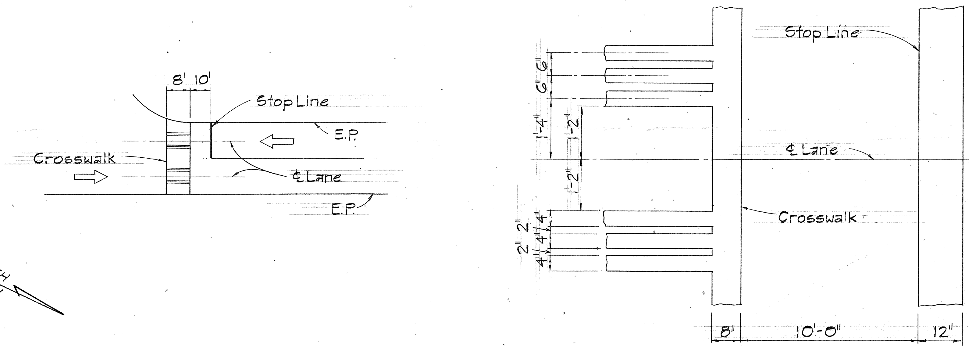
CROSSWALK & STOP LINE DETAIL Not To Scale
