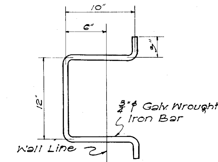
MANHOLE RUNG
