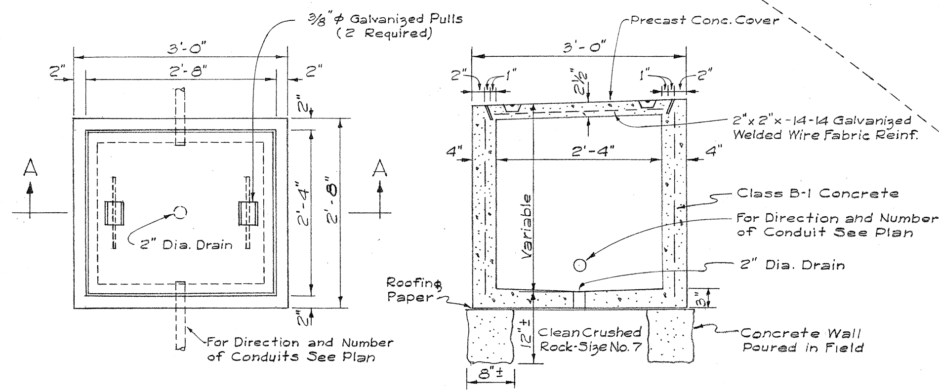
PLAN SECTION "A-A" DETAIL OF PULL BOX Scale: 3/4" = 1'-0"
