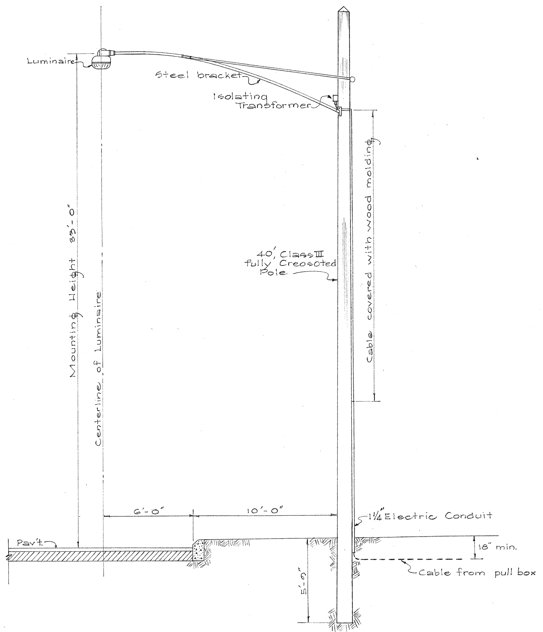
DETAIL OF 40' POLE Scale: 1/4" = 1'-0"
