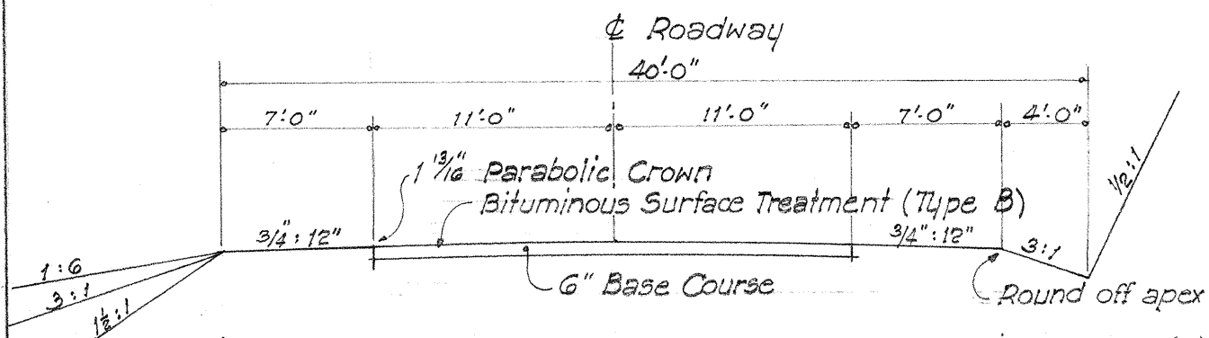
TYPICAL TANGENT SECTION - PROJS. FAP 21 B & FAP 7A(R)
