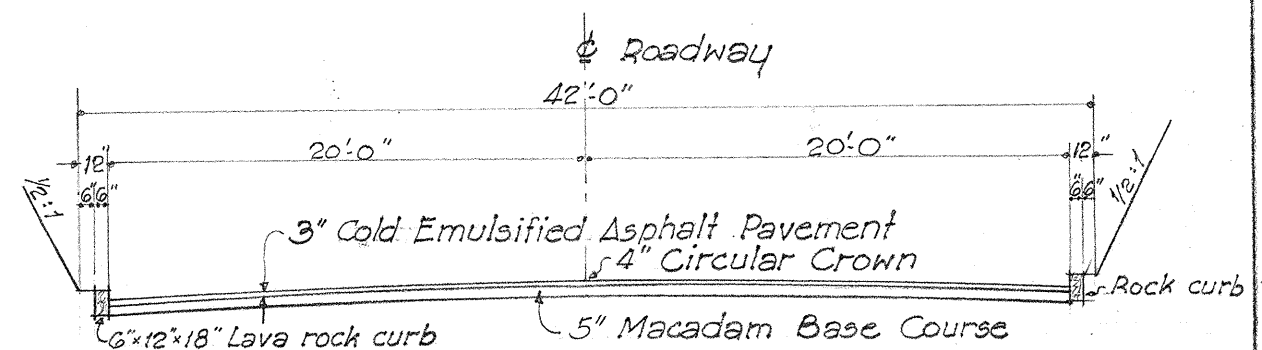
40' PAVEMENT TYPICAL TANGENT SECTION - PROJ. FAP 7-D
