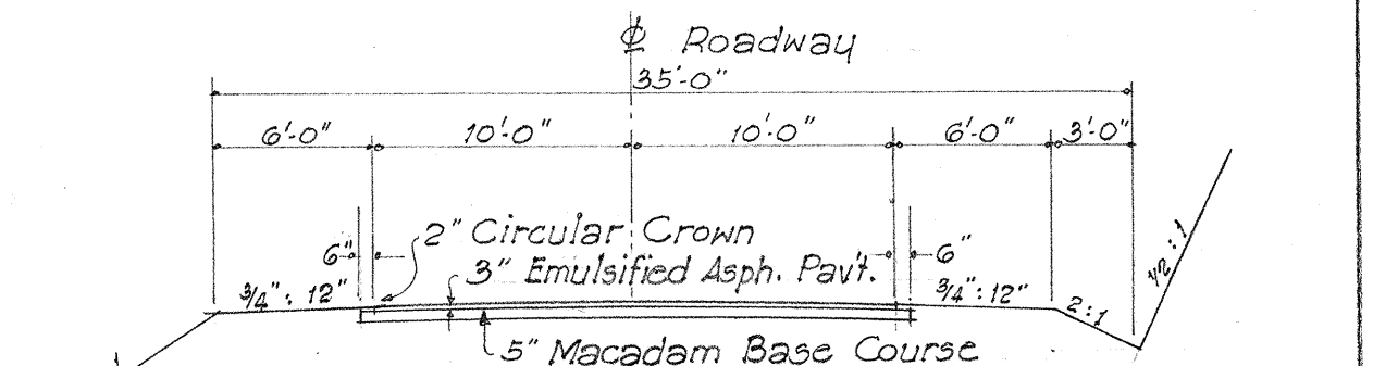
20' PAVEMENT TYPICAL TANGENT SECTION - PROJ. FAP 7-D
