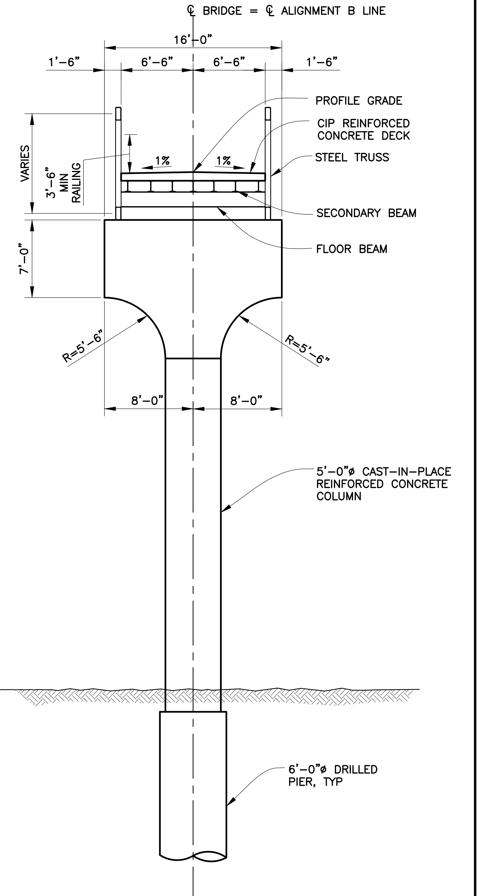
TYPICAL SECTION SCALE: 3/16"=1'-0"
