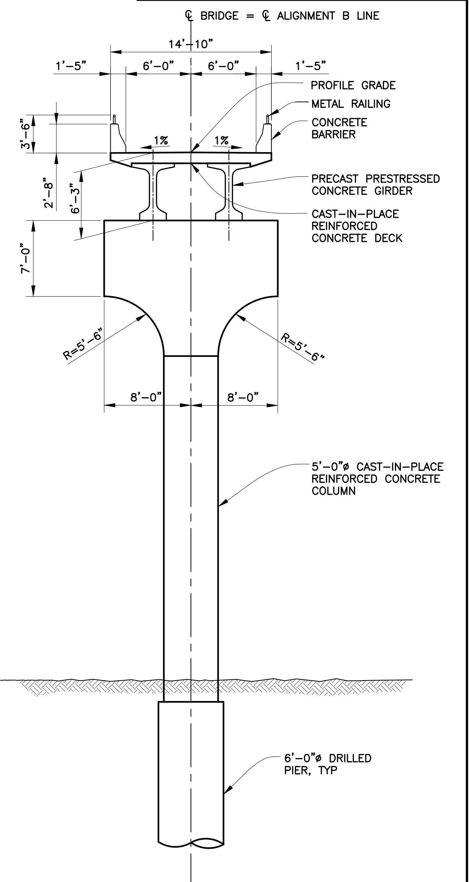
TYPICAL SECTION SCALE: 3/16"=1'-0" NOTE: FOR ILLUSTRATIVE PURPOSES ONLY.
