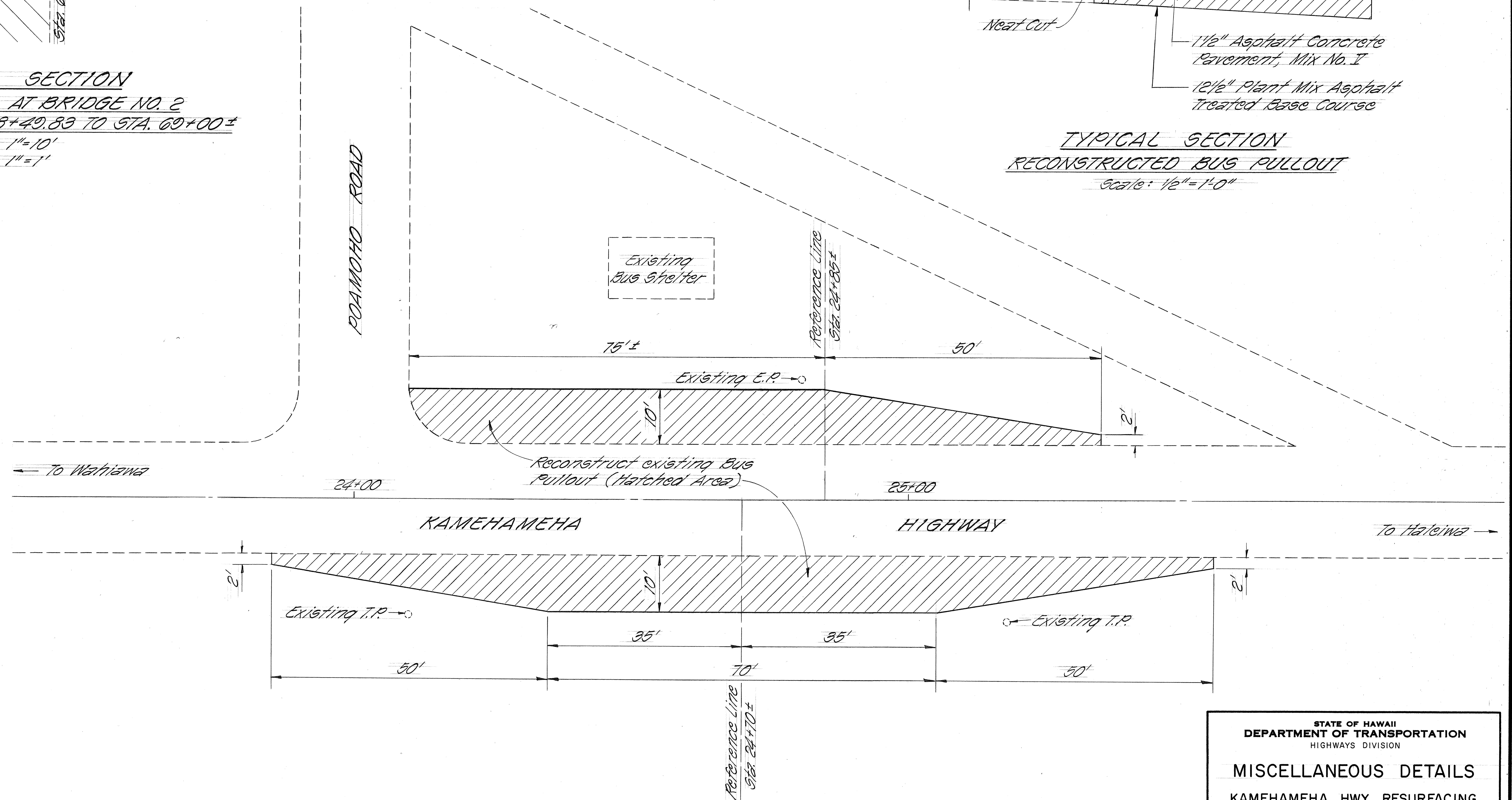
PLAN BUS PULLOUT RECONSTRUCTION DETAIL KAMEHAMEHA HWY. ~ STA. 24+70± RT. & STA. 24+85± LT. Scale: 1"=10'
