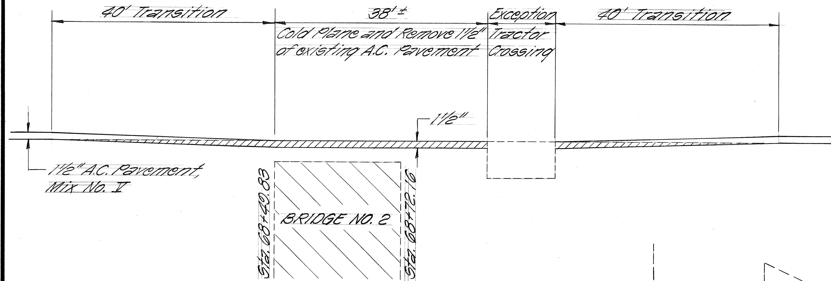
LONGITUDINAL SECTION COLD PLANING DETAIL AT BRIDGE NO. 2 KAMEHAMEHA HWY. ~ STA. 68+40.83 TO STA. 69+00± Scale: Horiz. 1"=10' Vert. 1"=1'
