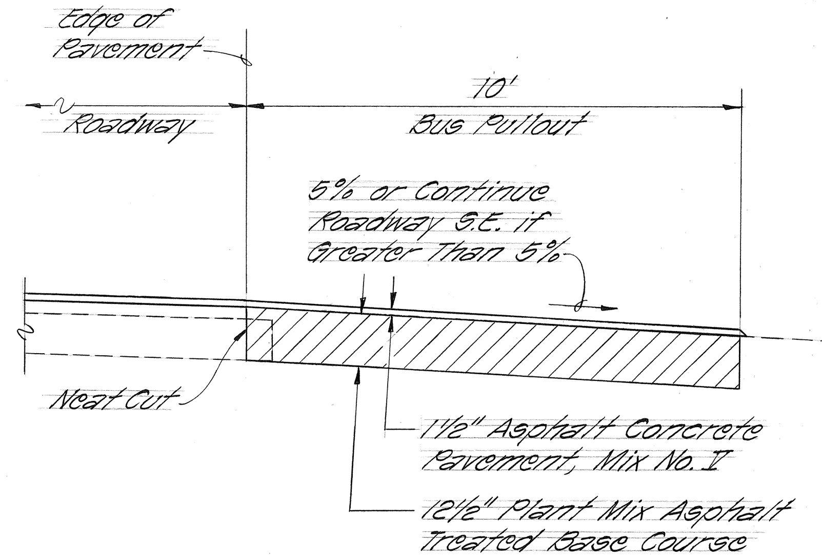
TYPICAL SECTION RECONSTRUCTED BUS PULLOUT Scale: 1/2"=1'-0"
