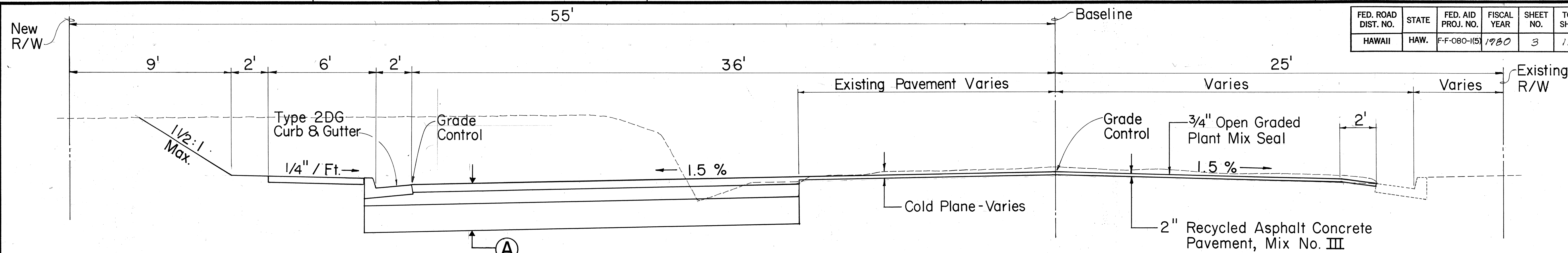
TYPICAL SECTION - KILANI AVE. TO HIWI PL. ± STA. 94+80 TO ± STA. 96+40
