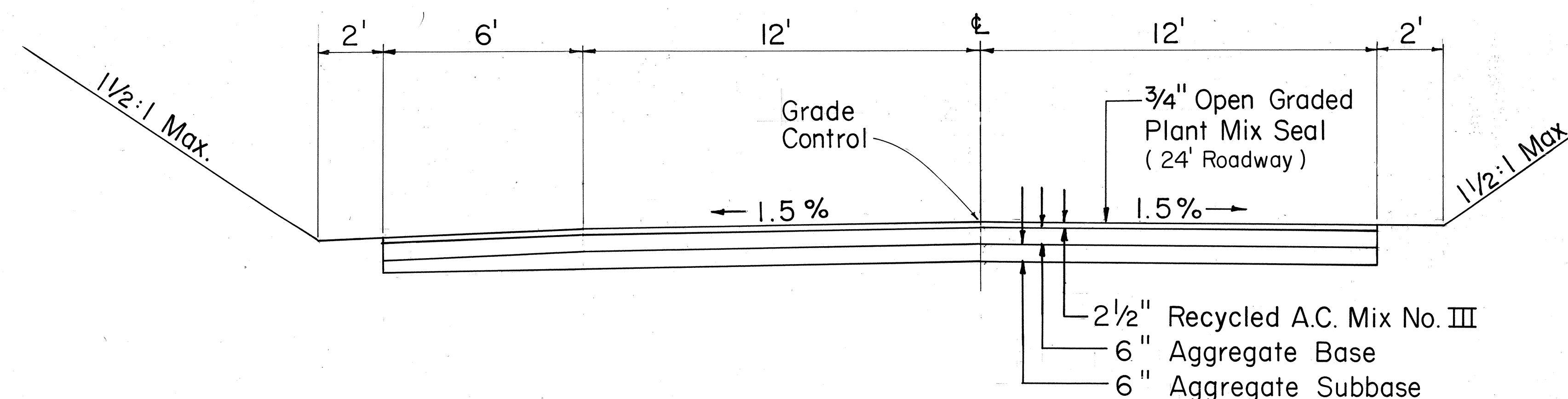
TYPICAL SECTION - HIWI PL. ± STA. 96+50
