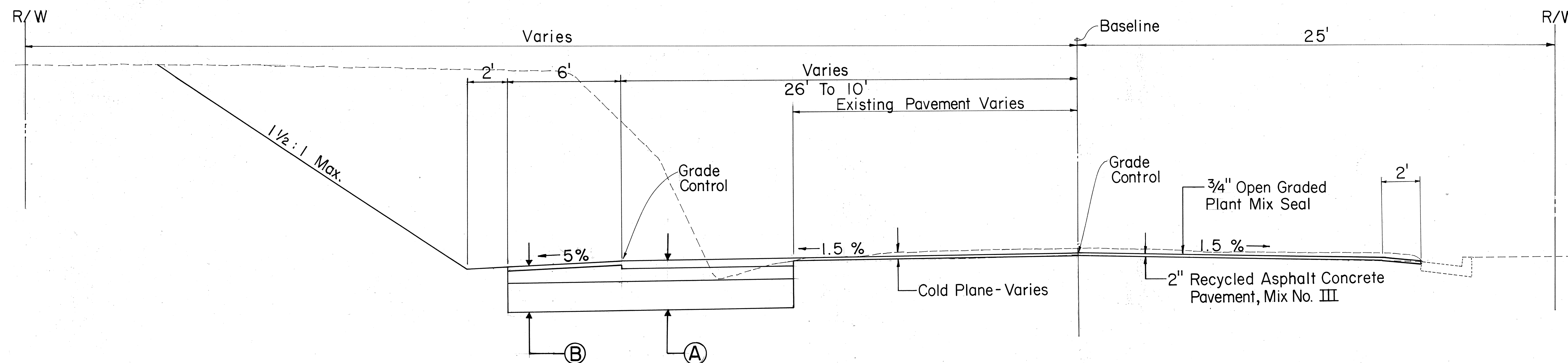
TYPICAL SECTION - HIWI PL. TO END OF PROJECT ± STA. 96+40 TO ± STA. 100+50
