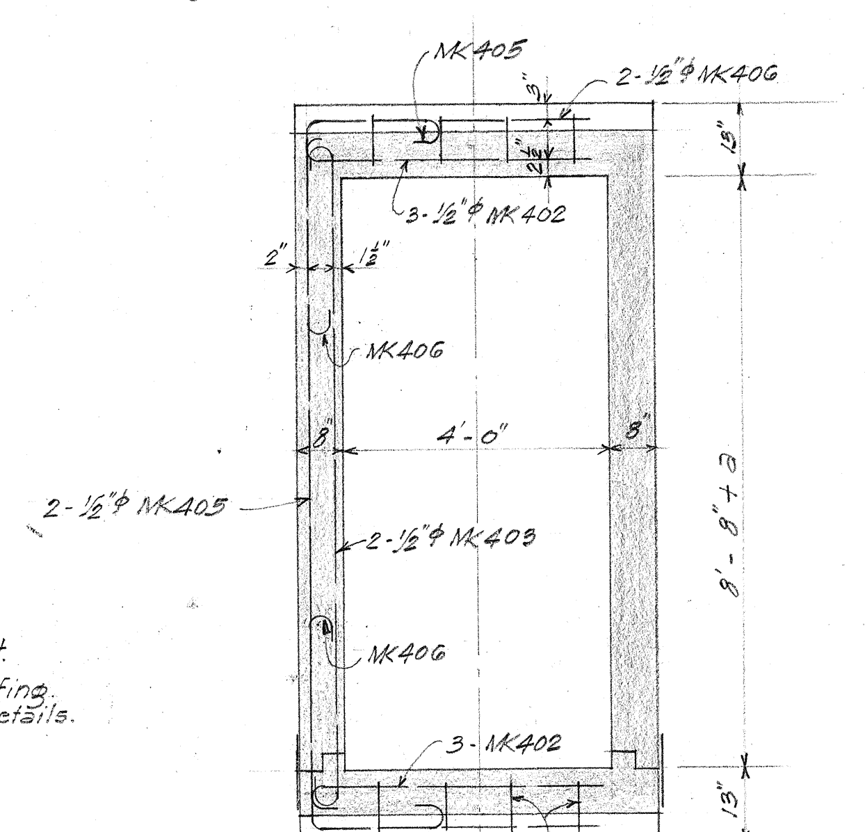
SECTION D-D 1/2" = 1'-0"
