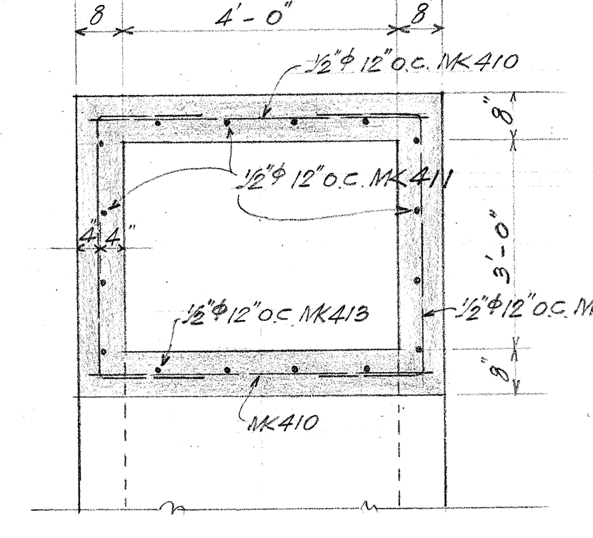
SECTION E-E 1/2" = 1'-0"
