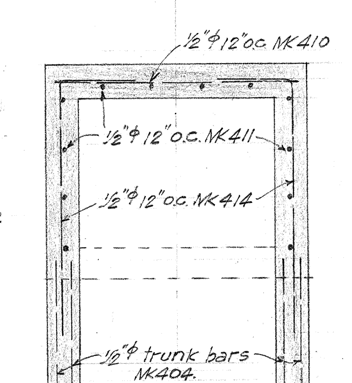
SECTION F-F 1/2" = 1'-0"
