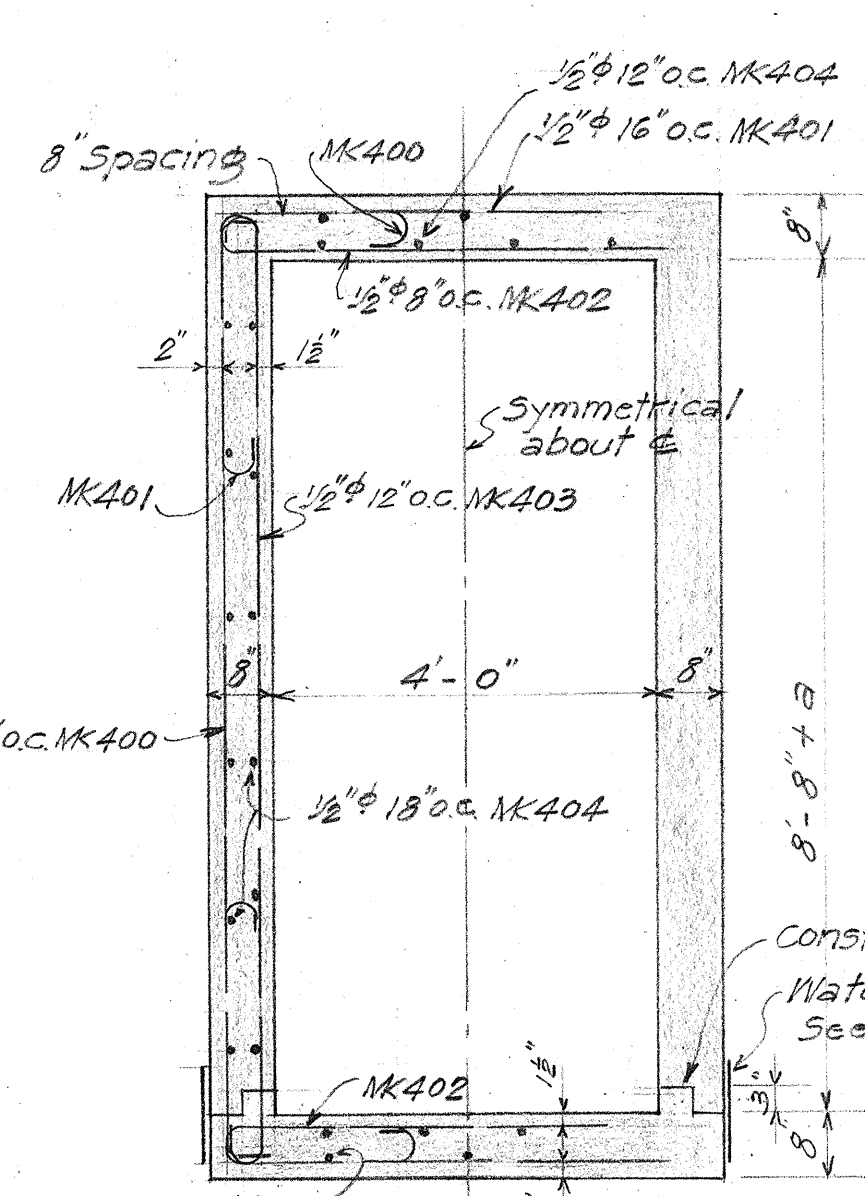
SECTION C-C 1/2" = 1'-0"
