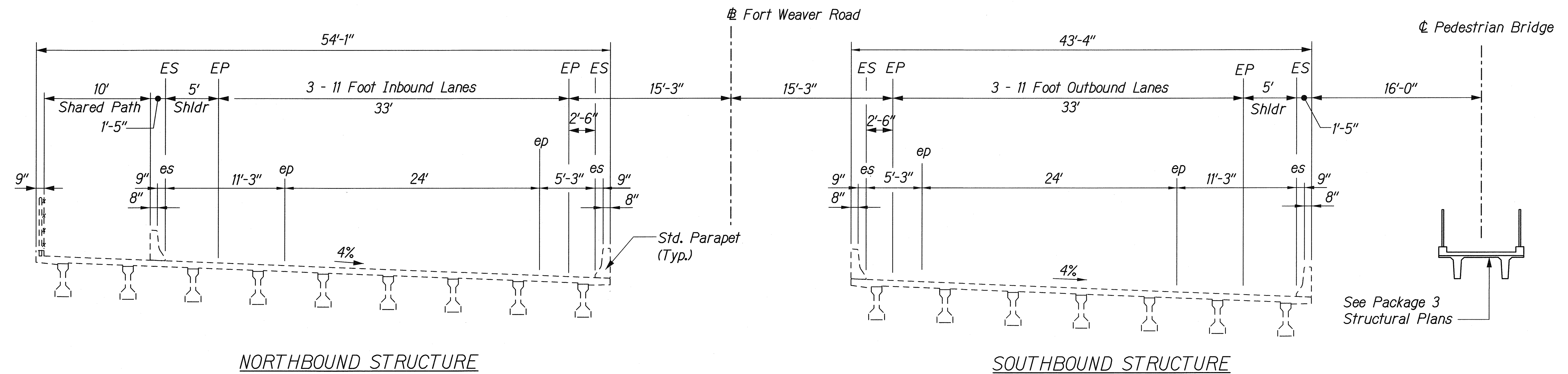
TYPICAL DECK SECTION - HONOLIULI BRIDGE FORT WEAVER ROAD
