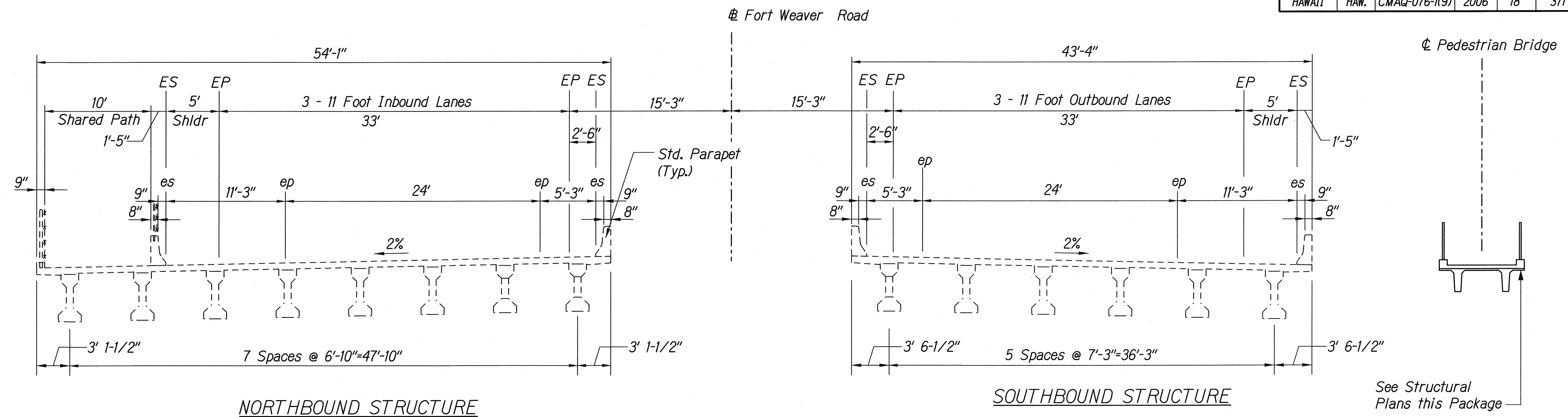
TYPICAL DECK SECTION - CANE HAUL ROAD OVERPASS BRIDGE FORT WEAVER ROAD
