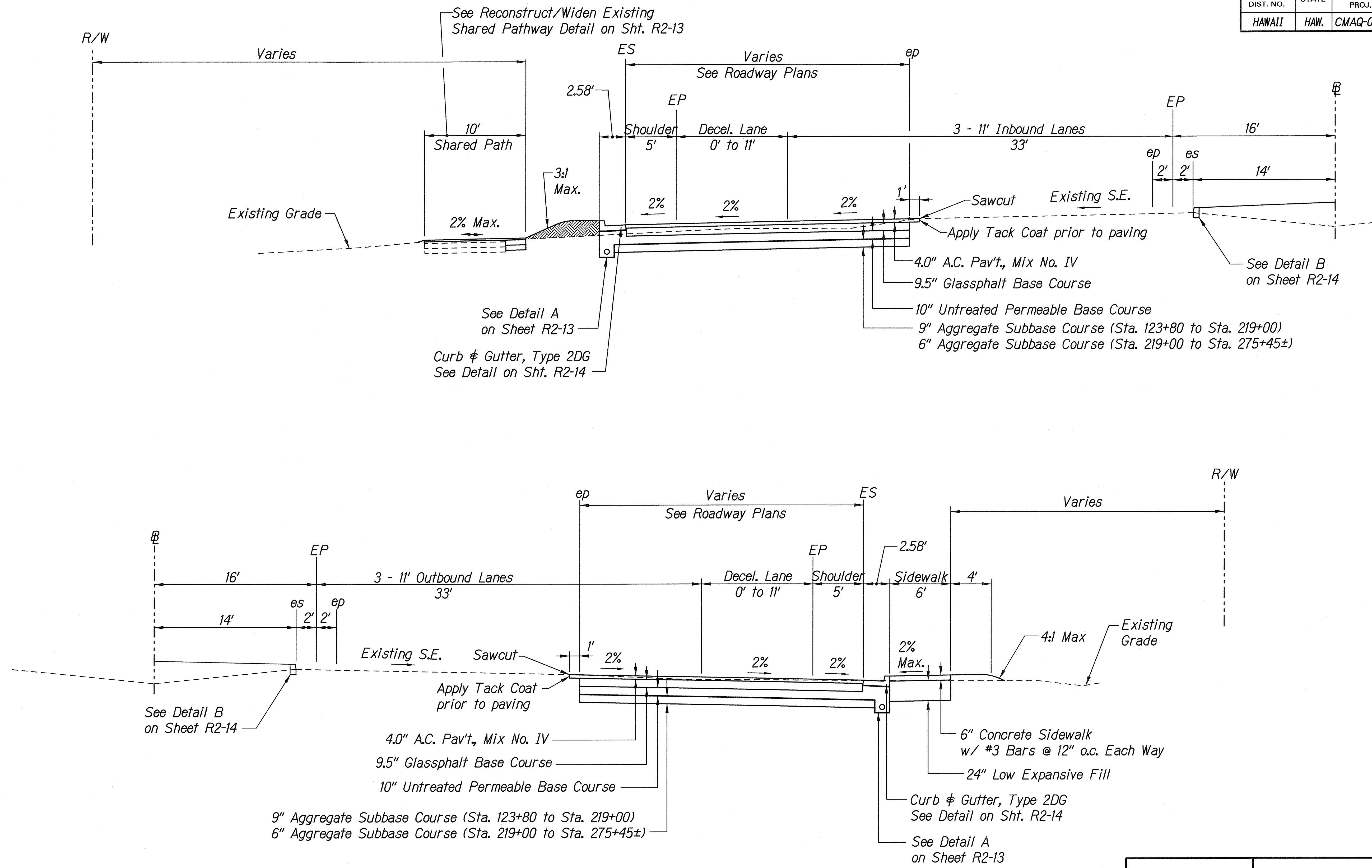
TYPICAL SECTION FORT WEAVER ROAD @ STA. 163+50 TO @ STA. 239+00 Scale: 1" = 5'
