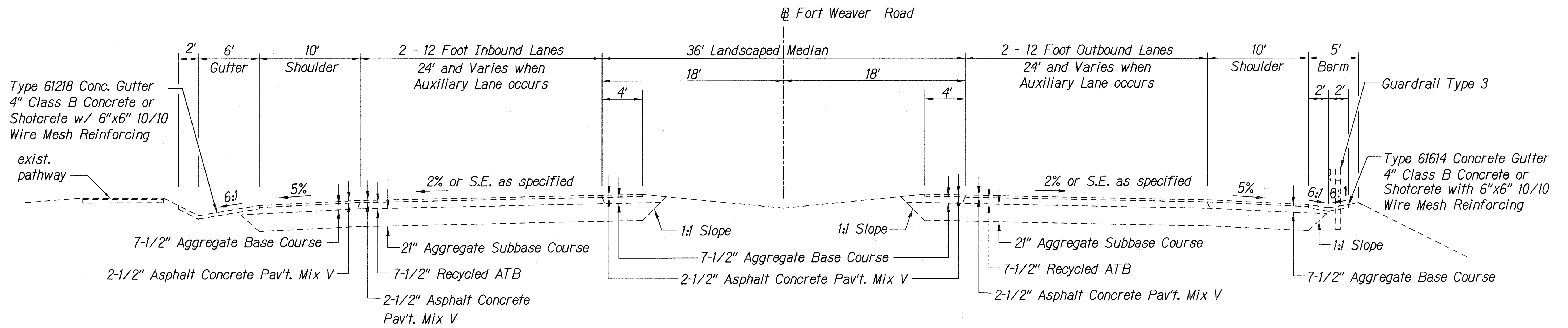
TYPICAL SECTION - EXISTING CONDITION - FORT WEAVER ROAD Scale: 1" = 5'
