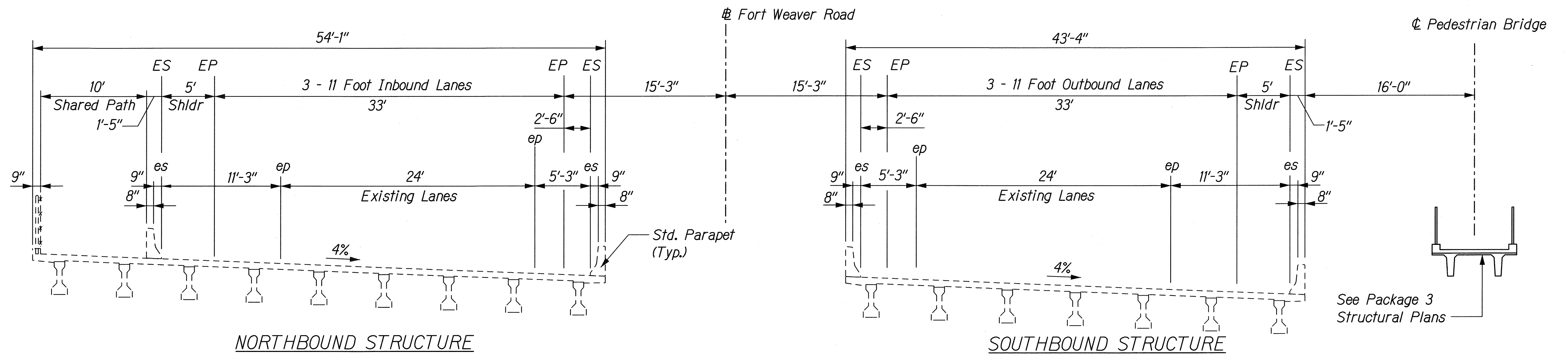
TYPICAL DECK SECTION - HONOUULIULI BRIDGE FORT WEAVER ROAD Scale: 1" = 5'
