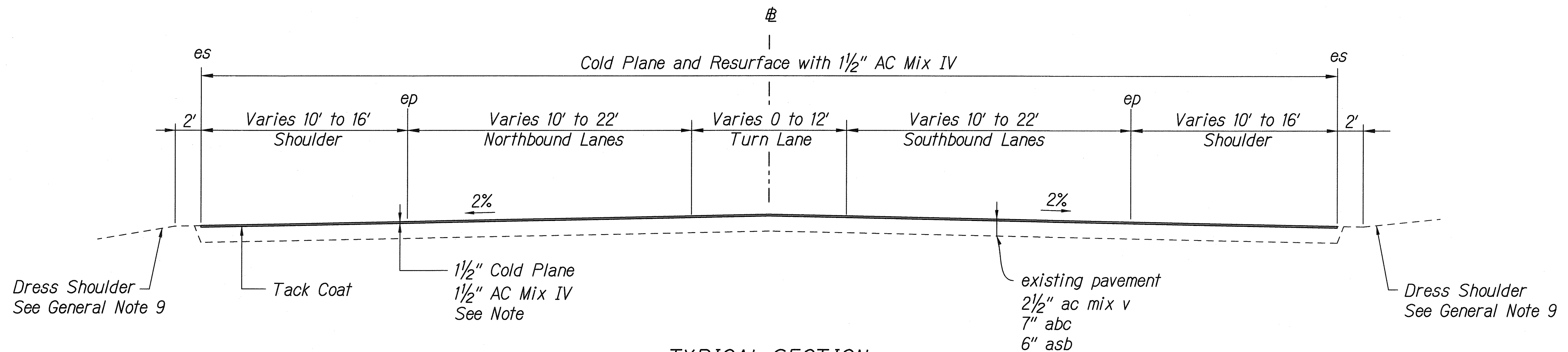
TYPICAL SECTION FORT WEAVER ROAD \pm STA. 74+70± TO \pm STA. 85+00± Scale: 1" = 5'
