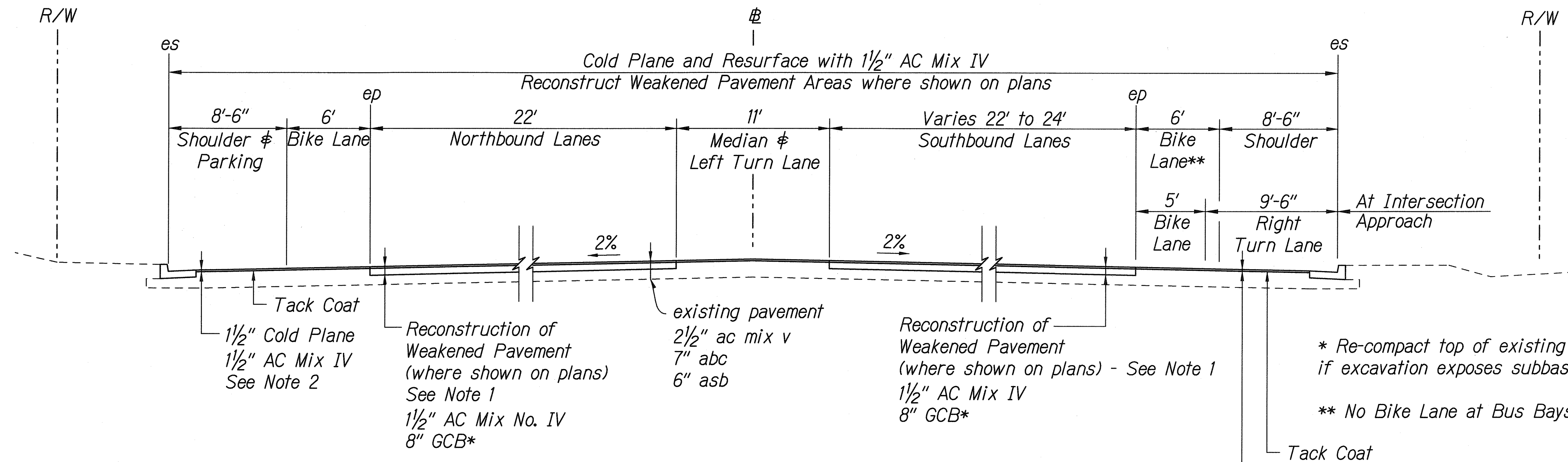
TYPICAL SECTION FORT WEAVER ROAD \pm STA. 7+52.58± TO \pm STA. 74+70± Scale: 1" = 5'
