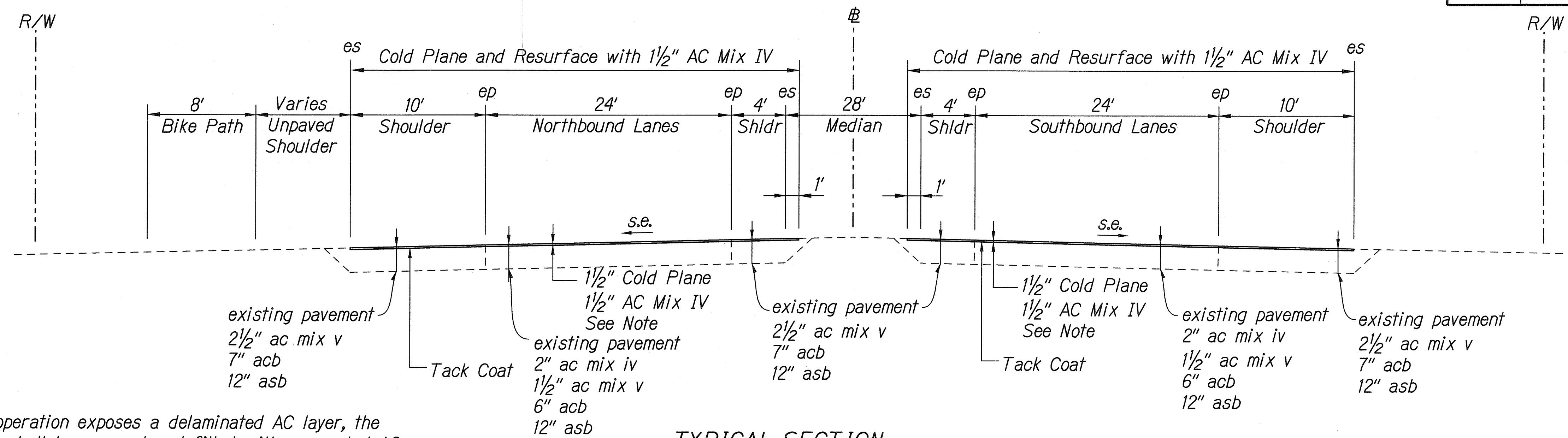
TYPICAL SECTION FORT WEAVER ROAD ± STA. 257+45 TO ± STA. 259+25± Scale: 1" = 5'
