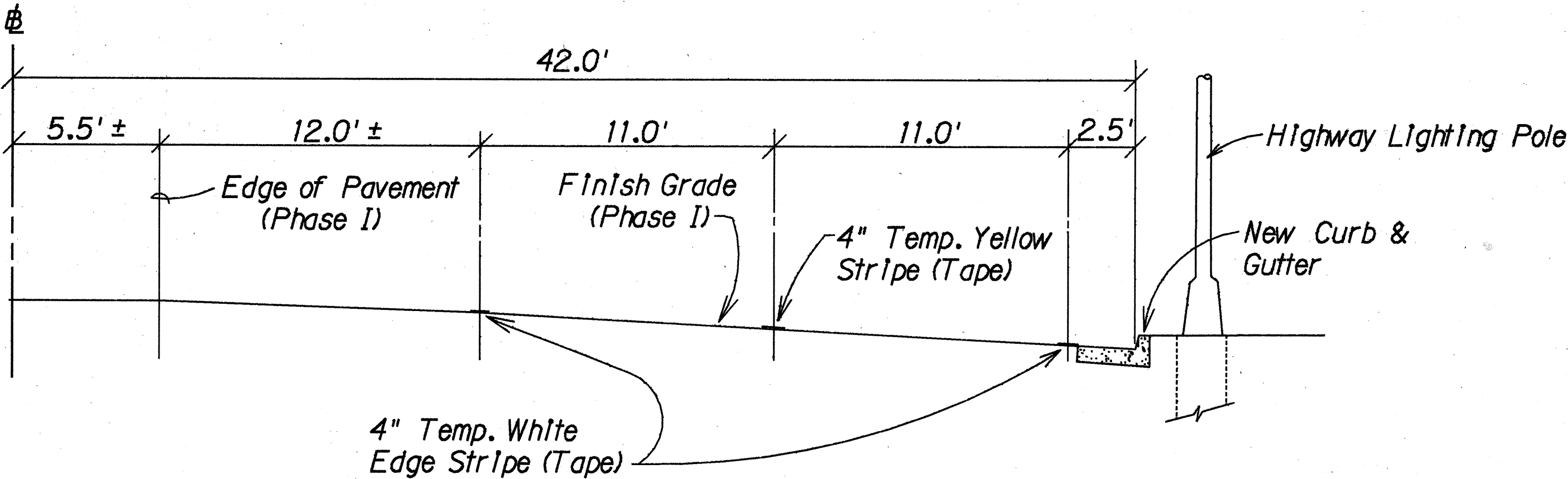
TYPICAL SECTION DETOUR ROAD - PHASE II Not To Scale
