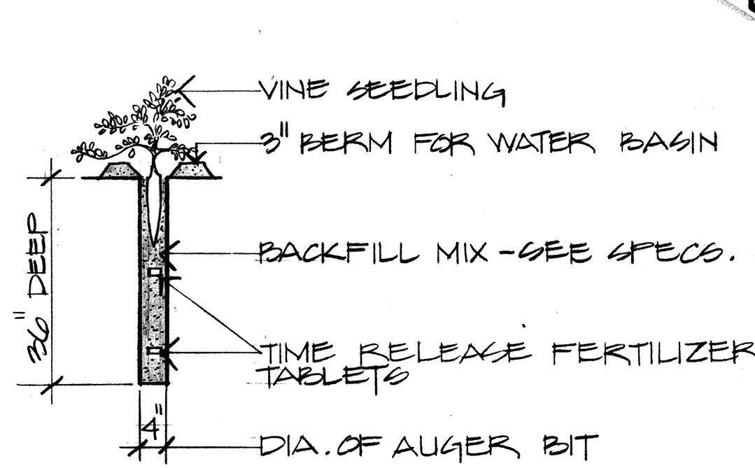
3 VINE PLANTING DETAIL NO SCALE (NOT IN CONTRACT)
