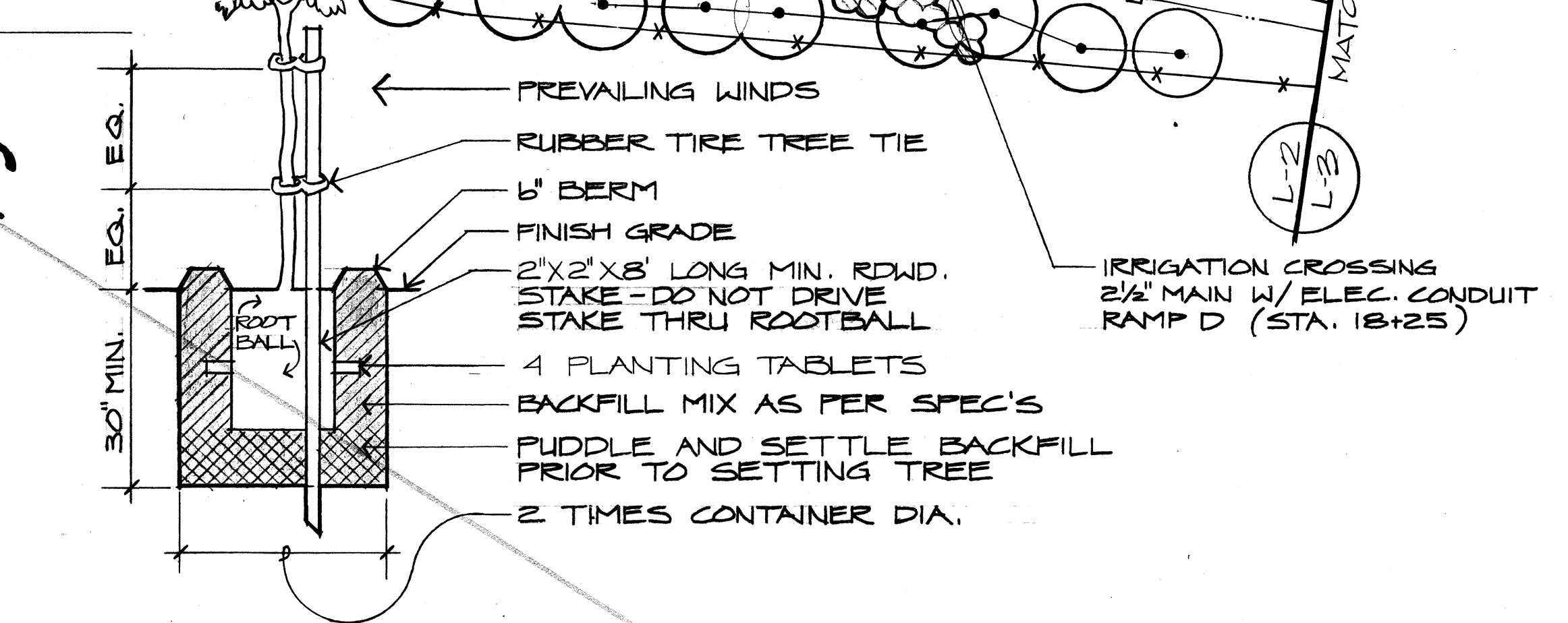
4 TREE PLANTING and STAKING DETAIL NO SCALE
