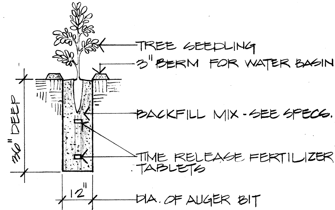
1 TREE PLANTING DETAIL NO SCALE
