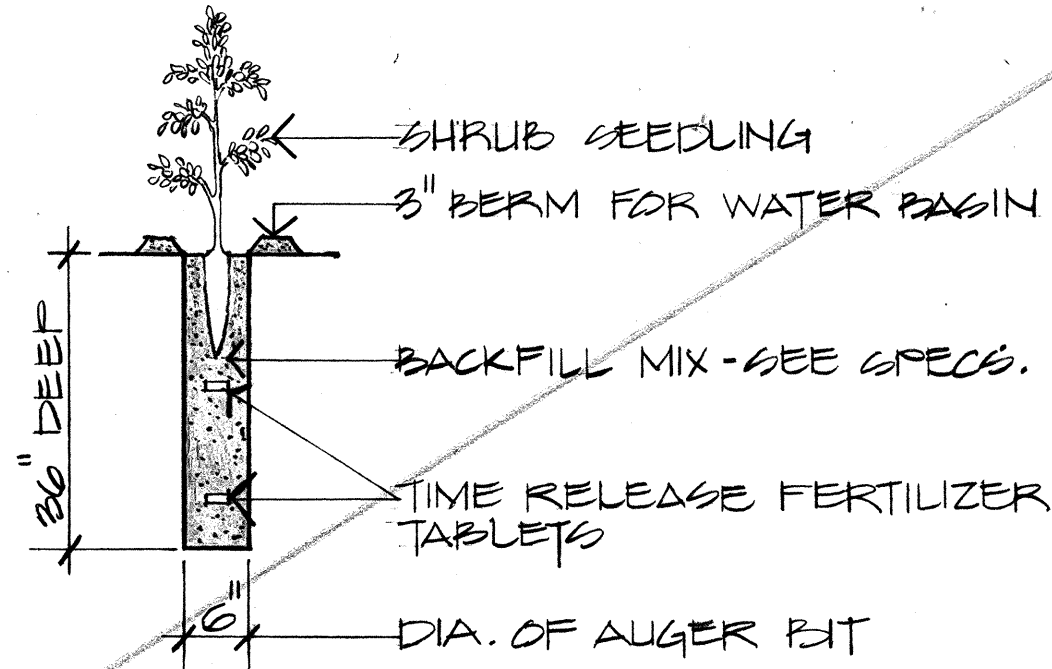
2 SHRUB PLANTING DETAIL NO SCALE
