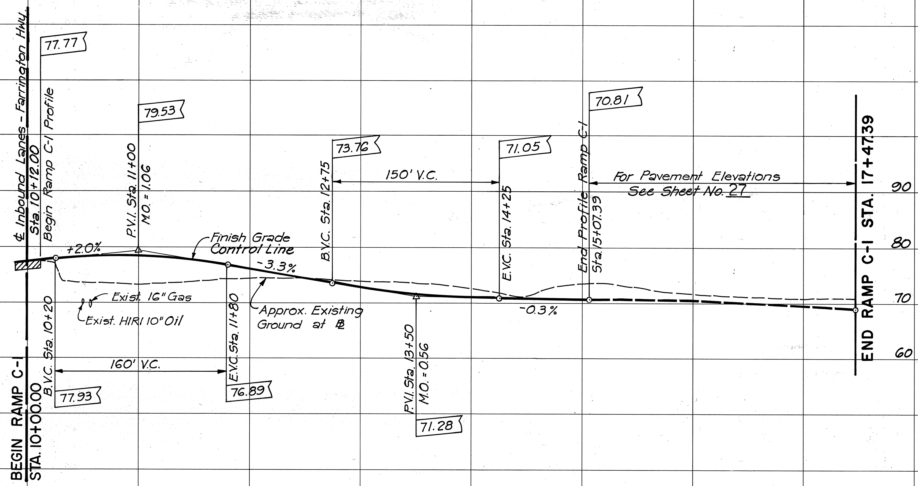
PROFILE SCALE: HOR. 1" = 50' VERT. 1" = 10' For Notes See Sheet No. 14
