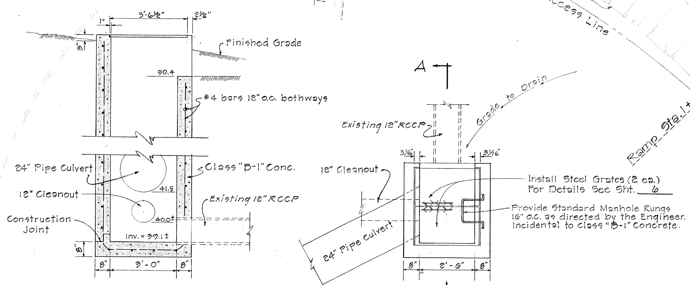
SECTION "A-A"
