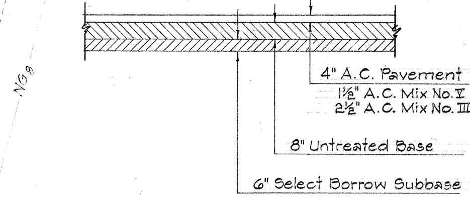
TYPICAL SECTION-FARRINGTON HIGHWAY Scale: 1/4" = 1'-0"
