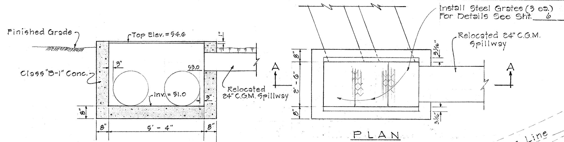
SECTION "A-A" DETAIL OF C.D.I. AT STA. 138+11 RIGHT
