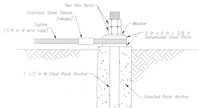
LATERAL ANCHOR CONNECTION DETAIL
