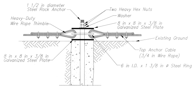
LATERAL ANCHOR CONNECTION DETAIL
