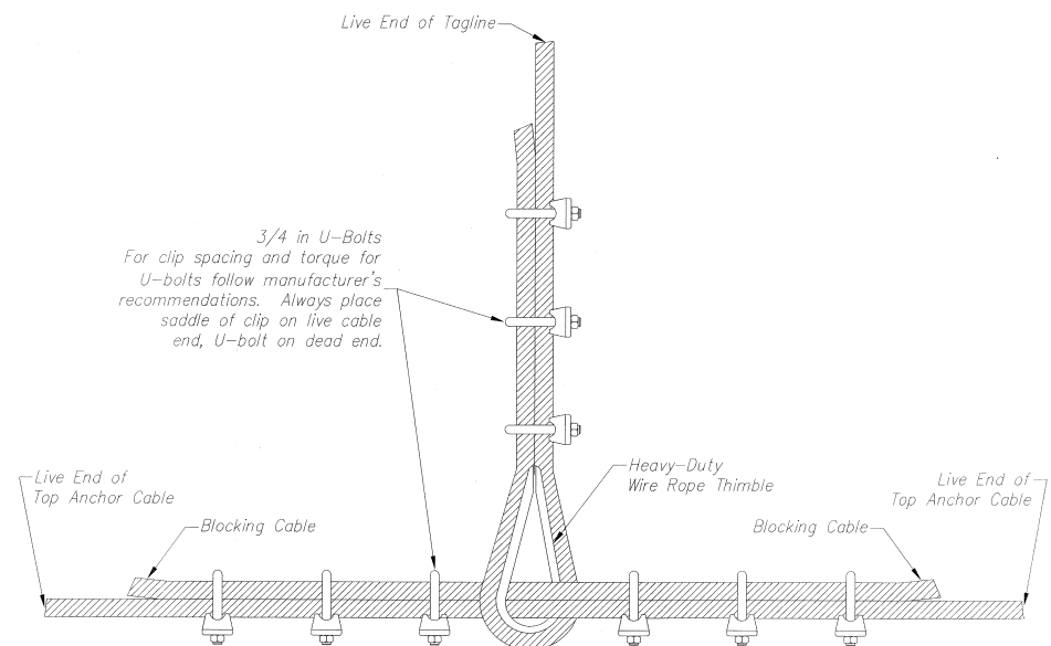
TAGLINE CONNECTION DETAILS
