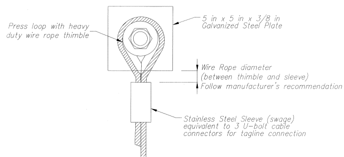
TRAP PLATE ANCHOR DETAIL
