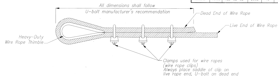
3/4 IN WIRE ROPE CLIP LOOP
