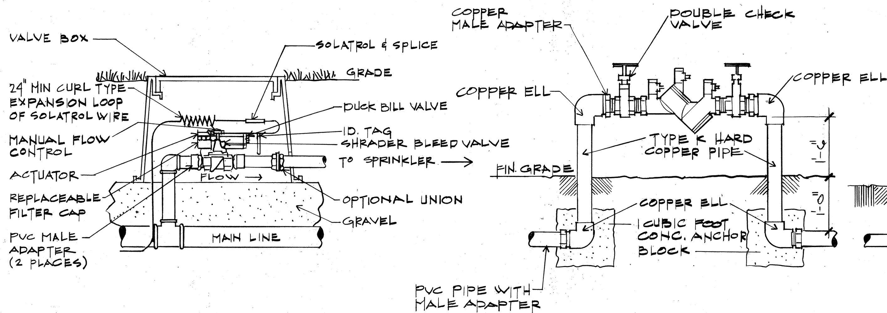
REMOTE CONTROL VALVE
