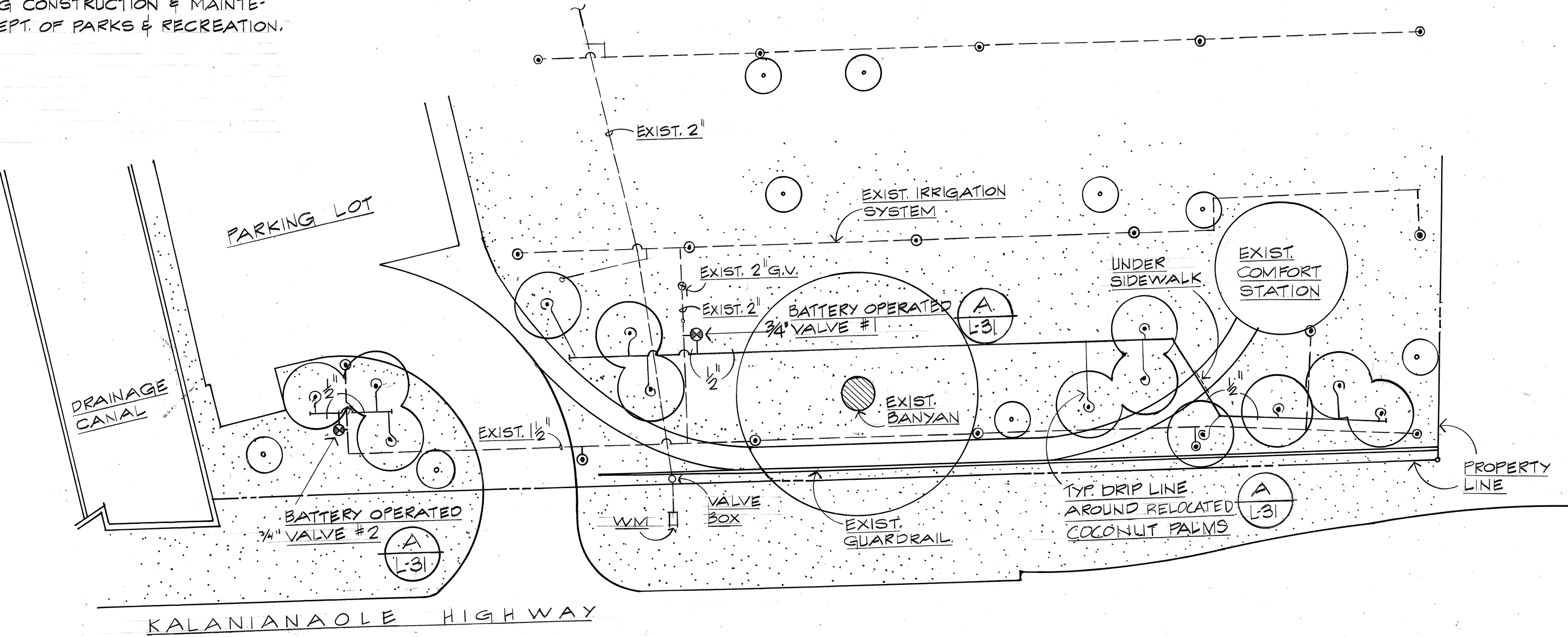
WAILUPE BEACH PARK / IRRIGATION PLAN SCALE = 1" = 20'
