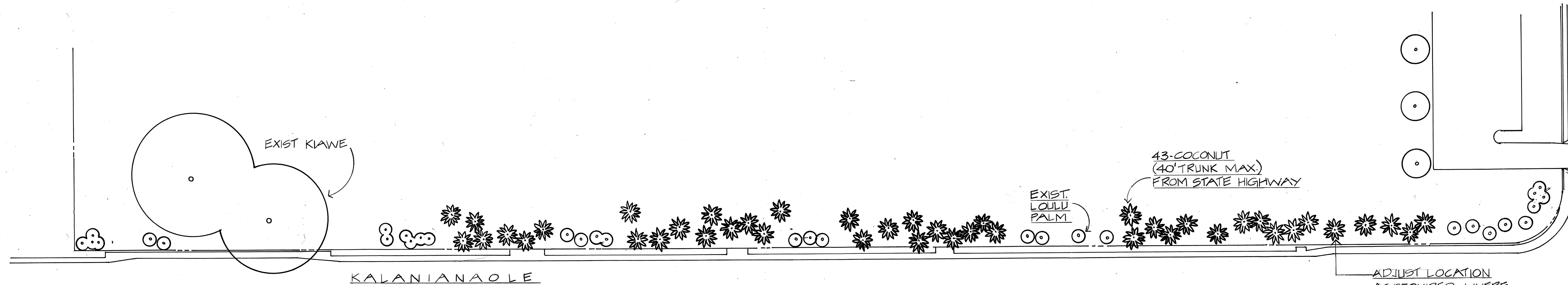
WAIALAE-IKI PLAYGROUND / PLANTING PLAN SCALE = 1"=40'
