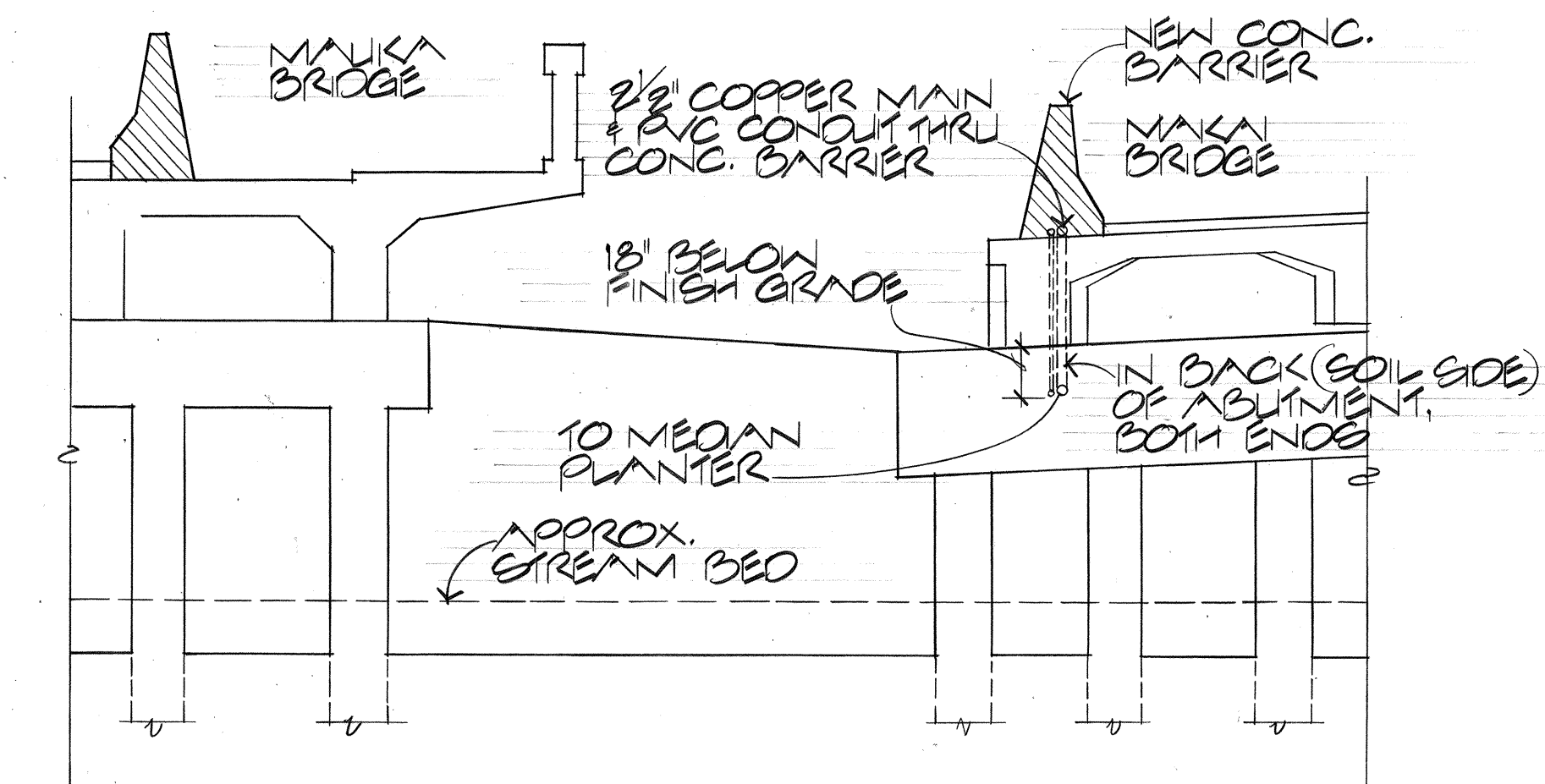
COPPER MAIN & PVC CONDUIT DETAIL NO SCALE
