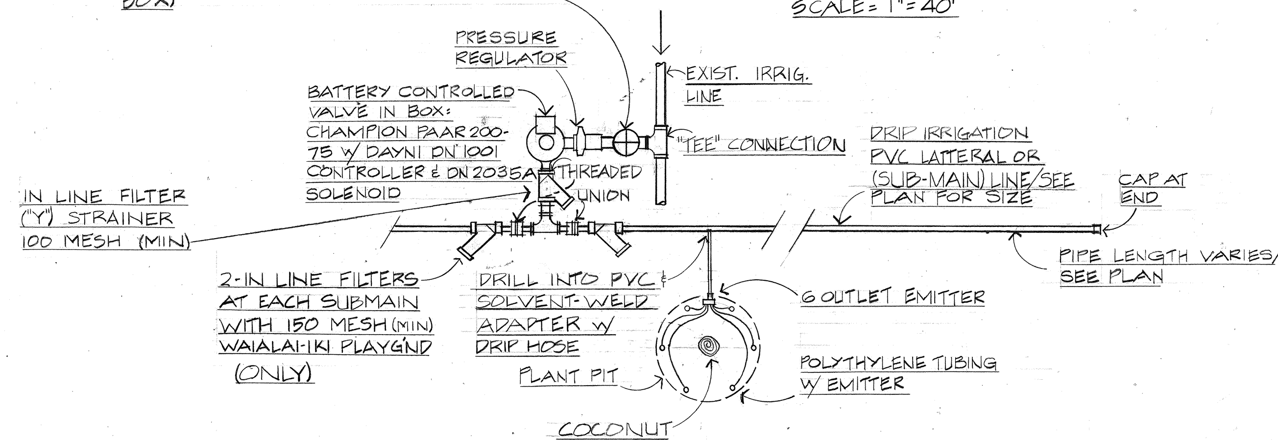
DRIP IRRIGATION-TYPICAL LAYOUT NO SCALE
