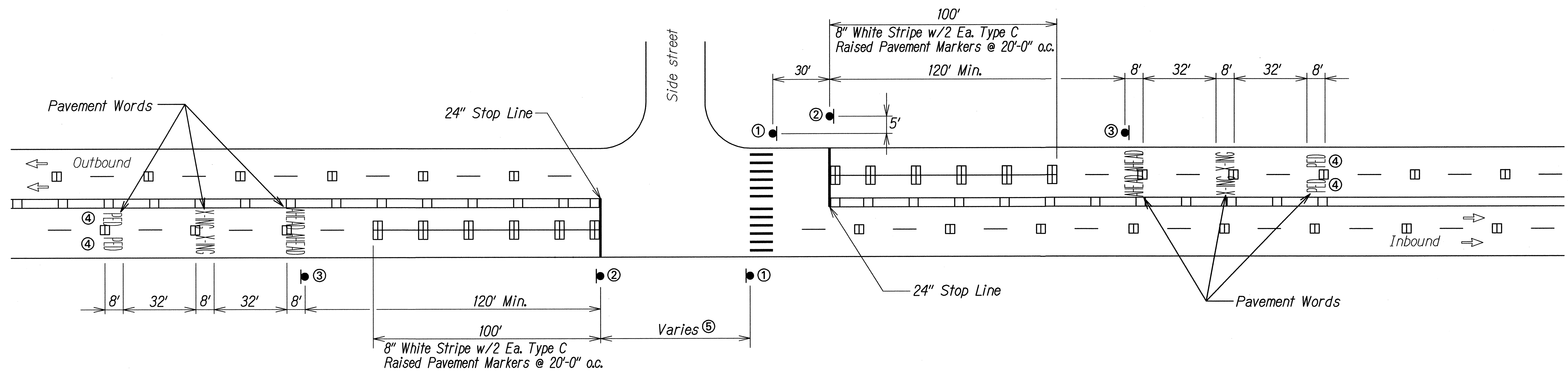
TYPICAL UNSIGNALIZED INTERSECTION MARKINGS (NO LEFT TURN STORAGE LANES) Not to Scale
