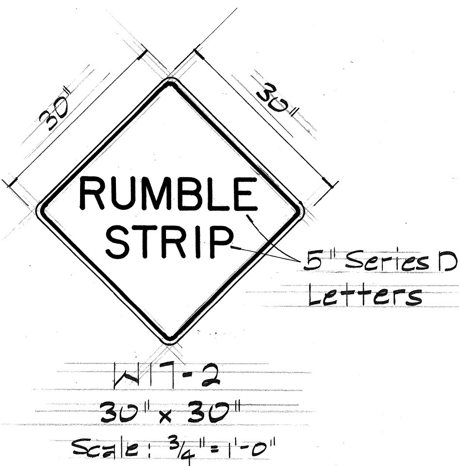
WARNING SIGN W17-2
