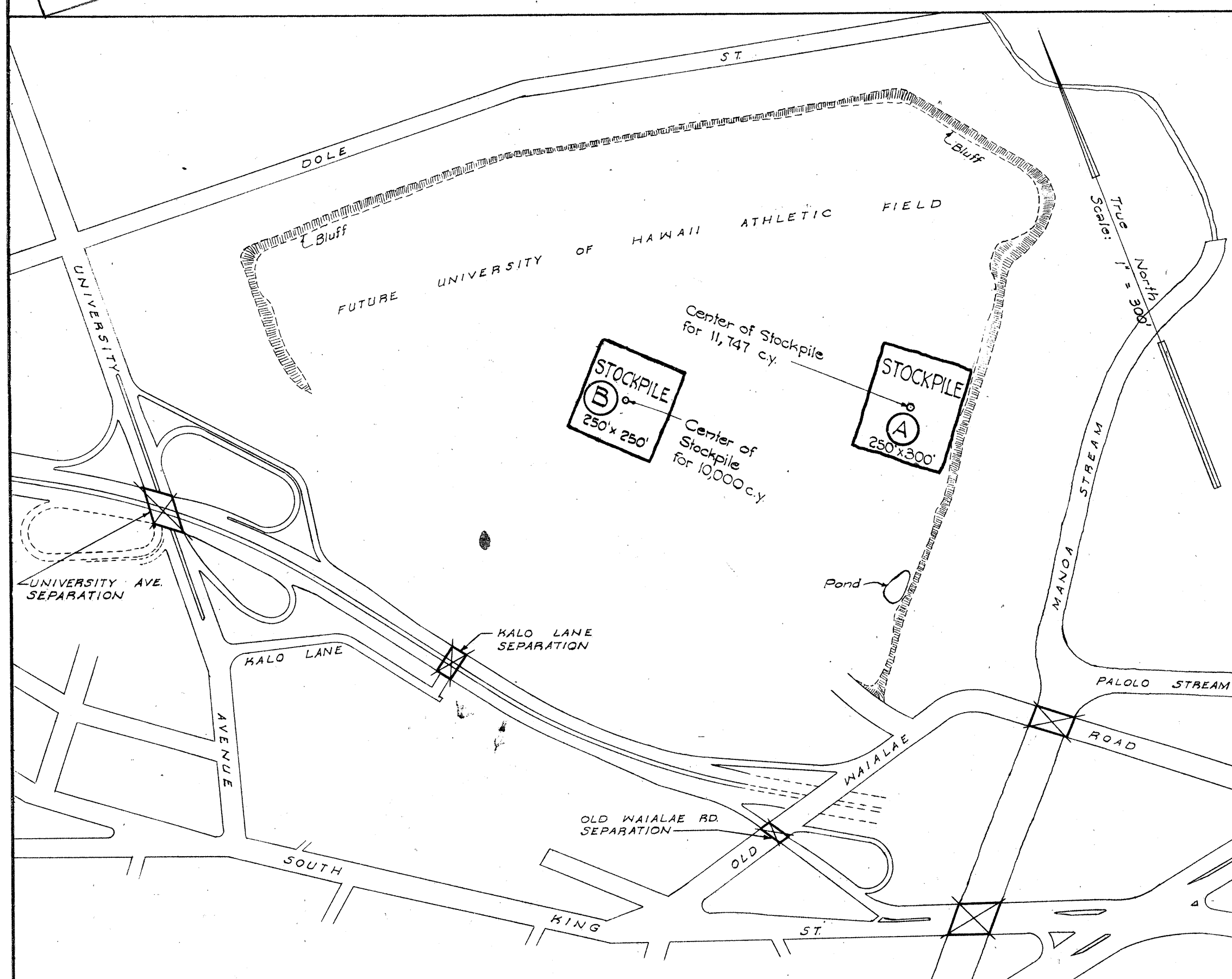
LOCATION PLAN SHOWING STOCKPILING SITE (Topsoil)
