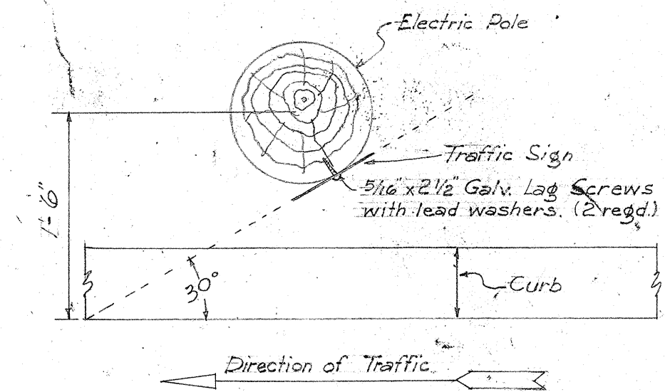
DETAIL SHOWING ANGLE OF TRAFFIC SIGNS AND CURB LINE Scale: 1" = 1'-0" (Above detail applies to "R-18" only)
