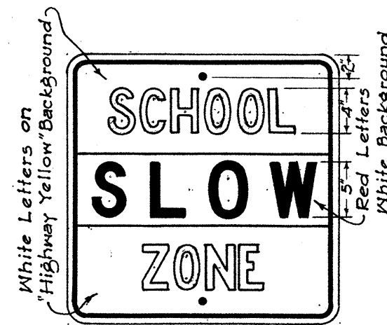
R-41-S 24" x 24"
