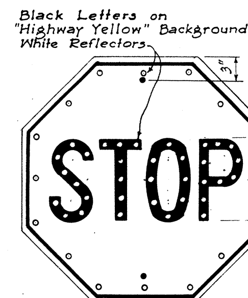
R-1 30" x 30"
