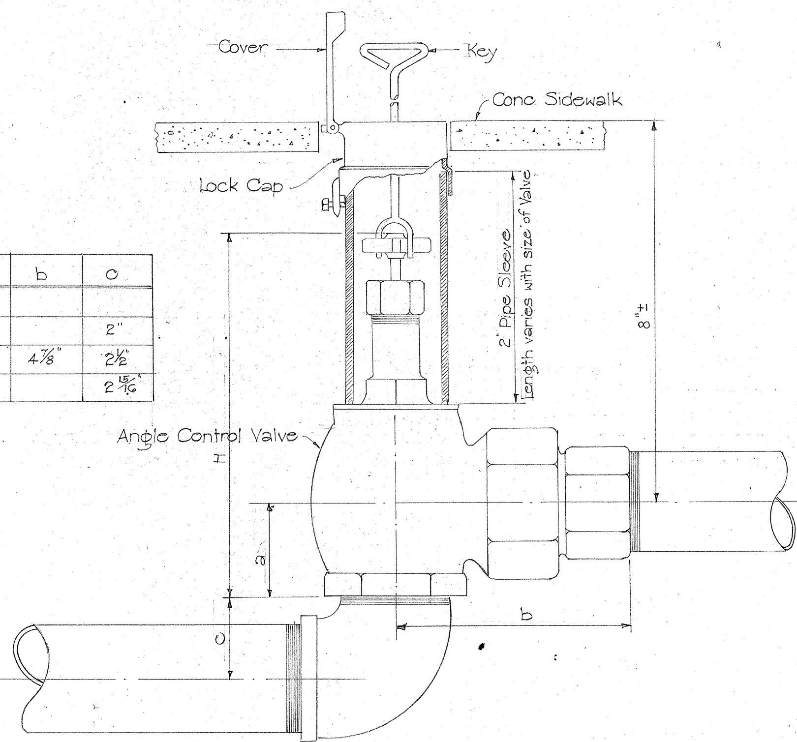
DETAIL OF ANGLE CONTROL VALVE, HOUSING, AND CAP.
