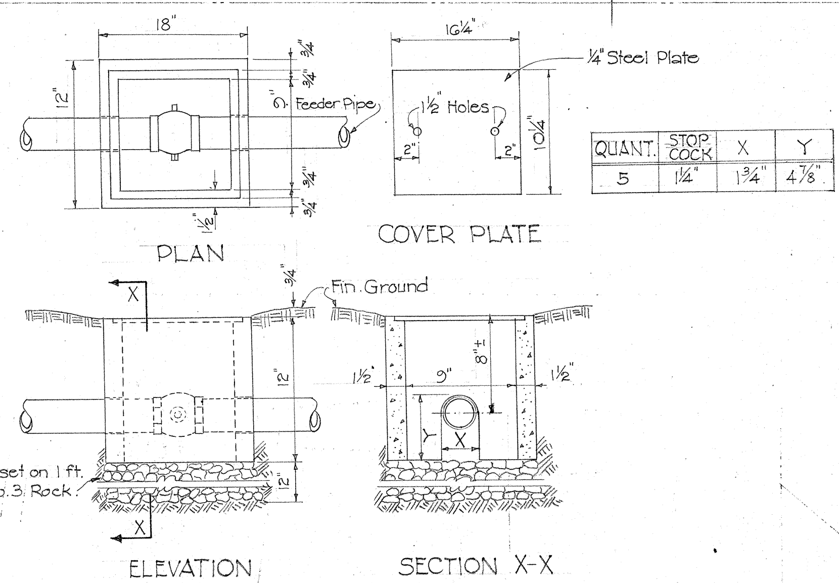
PRECAST CONCRETE BOX FOR STOPCOCKS Not to Scale
