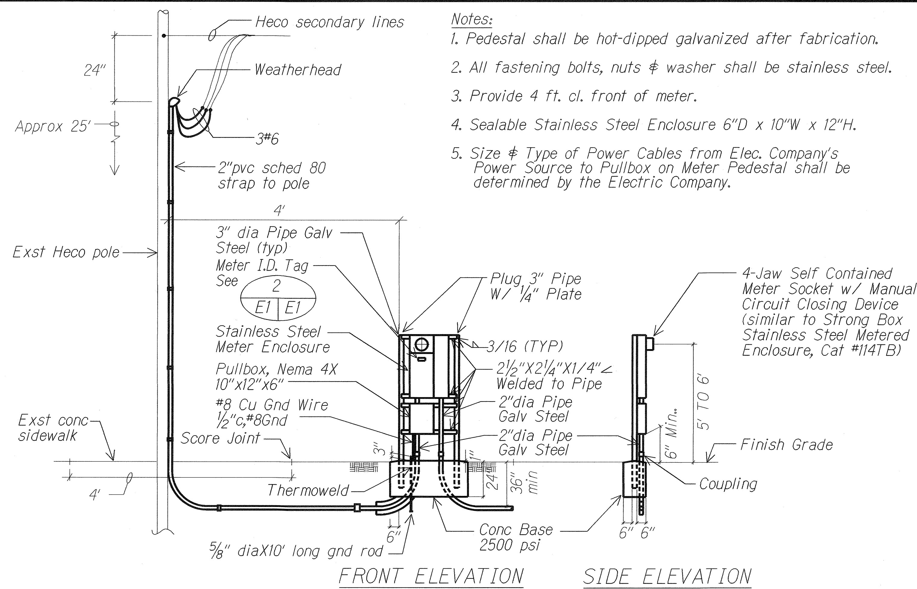
1 METER PEDESTAL FOR UNDERGROUND SERVICE
