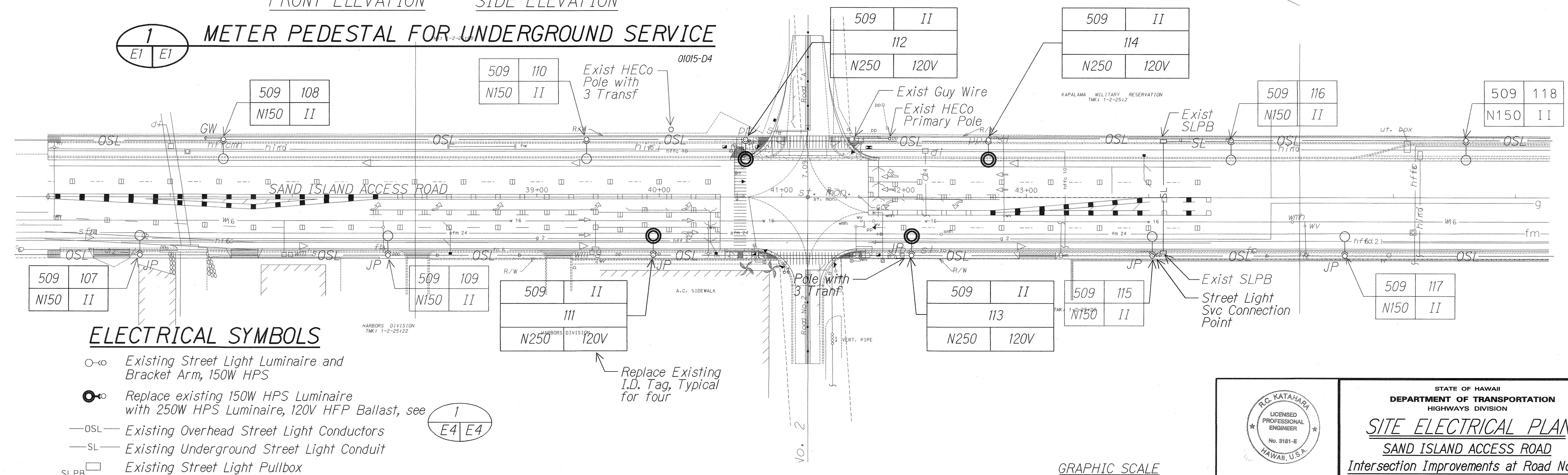
SITE ELECTRICAL PLAN SCALE: 1" = 40'-0" 01015-SB
