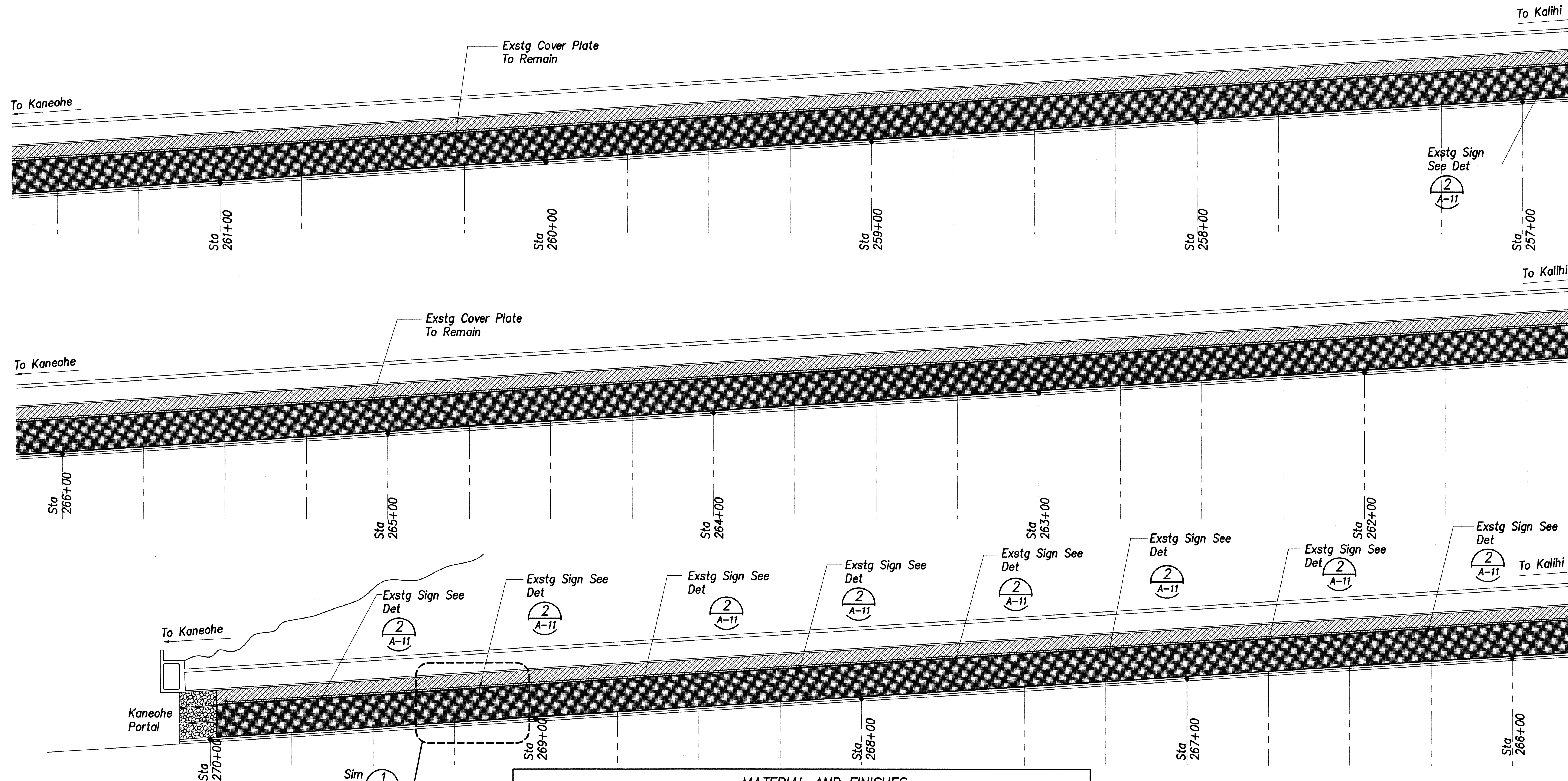
KANEOHE TUNNEL SOUTH WALL ELEVATION SCALE: 1/16" = 1'-0"
