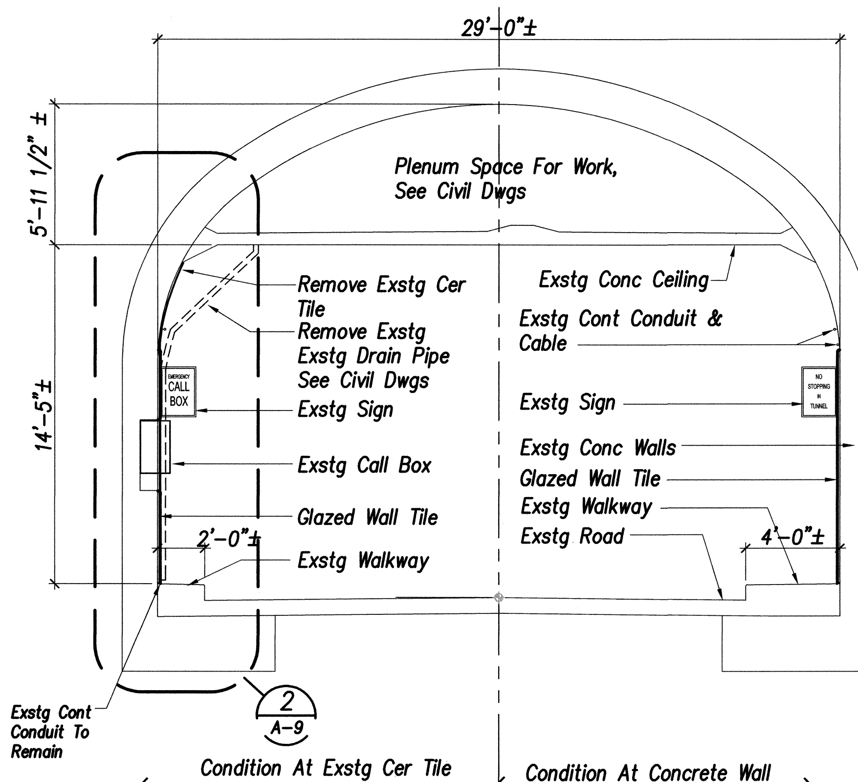
B KALIHI TUNNEL CROSS-SECTION SCALE: 1/4" = 1'-0"
