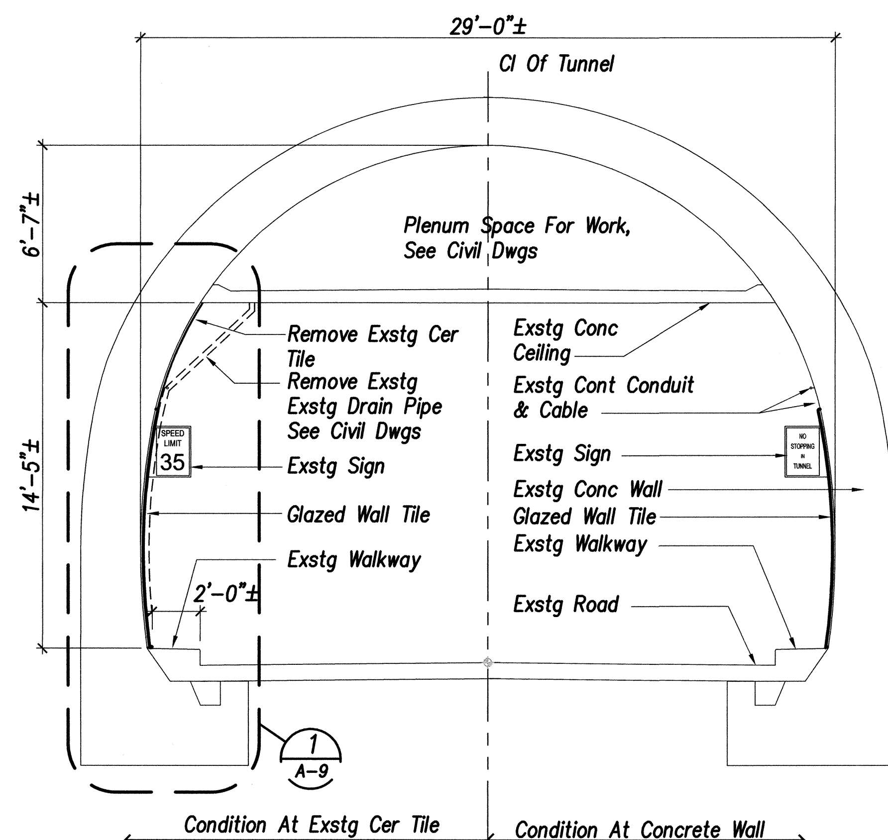
A KANEHOE TUNNEL-CROSS SECTION SCALE: 1/4" = 1'-0"
