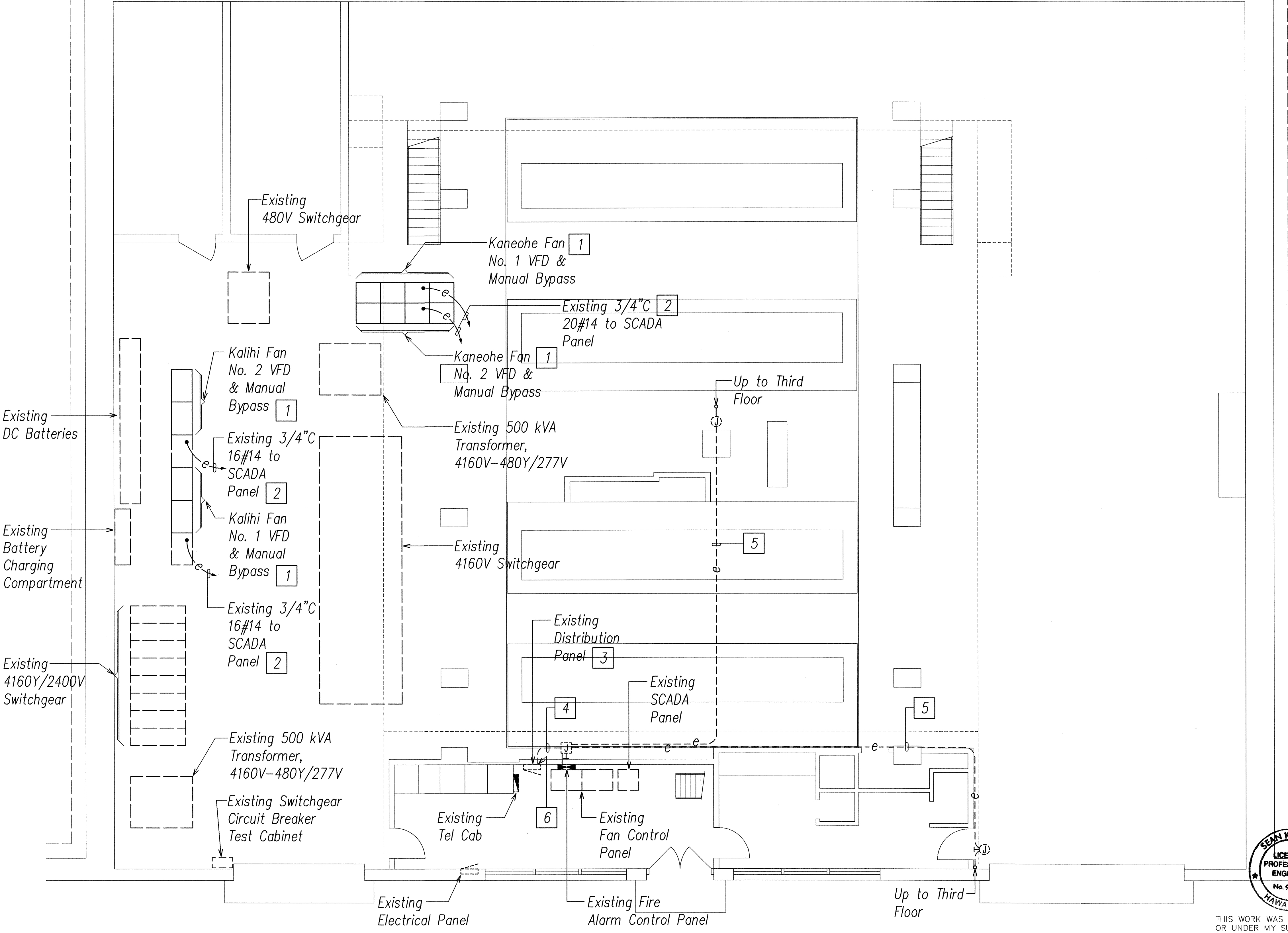
GROUND FLOOR ELECTRICAL PLAN SCALE: 3/16"=1'-0"
