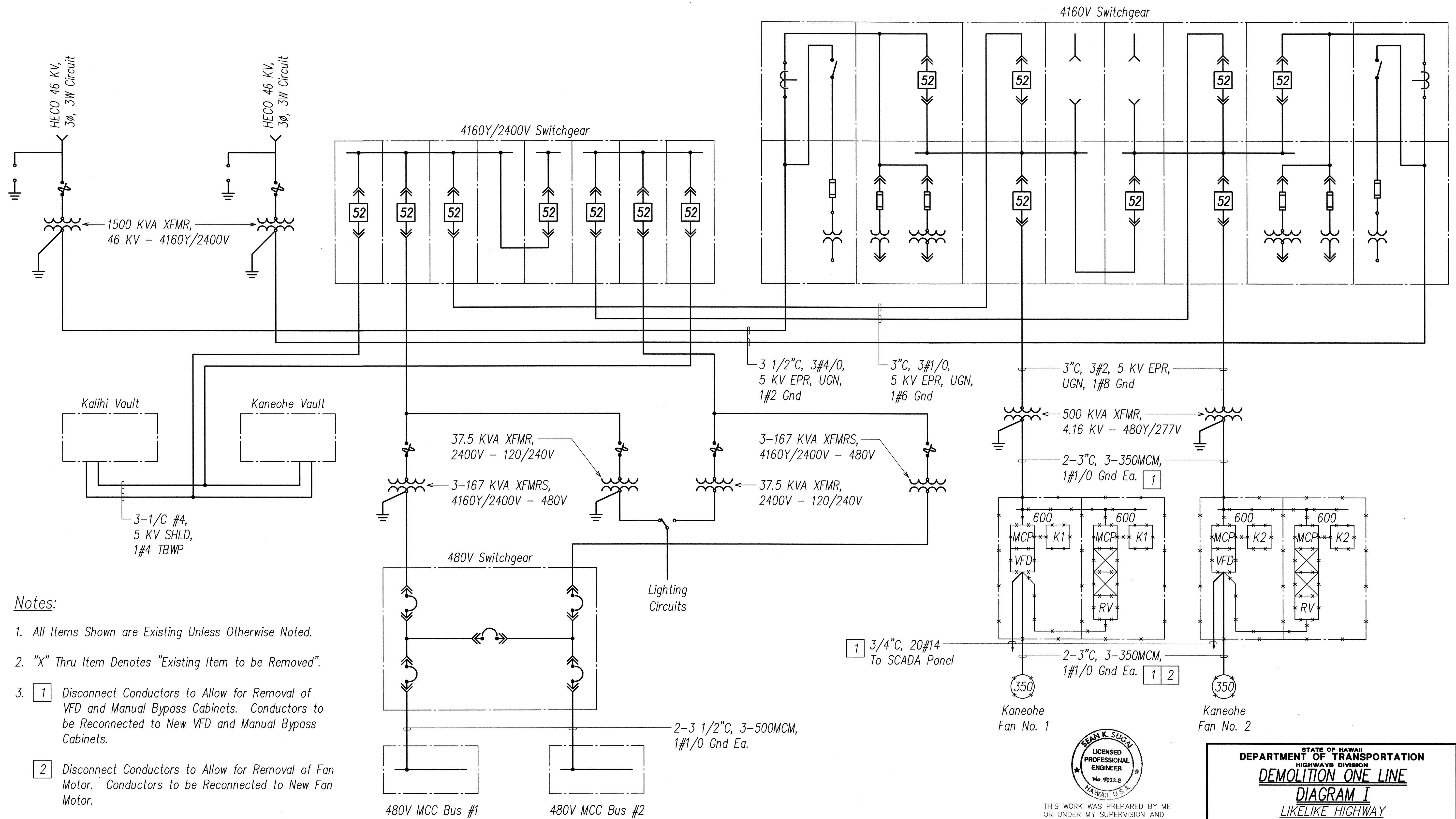
DEMOLITION ONE LINE DIAGRAM I
