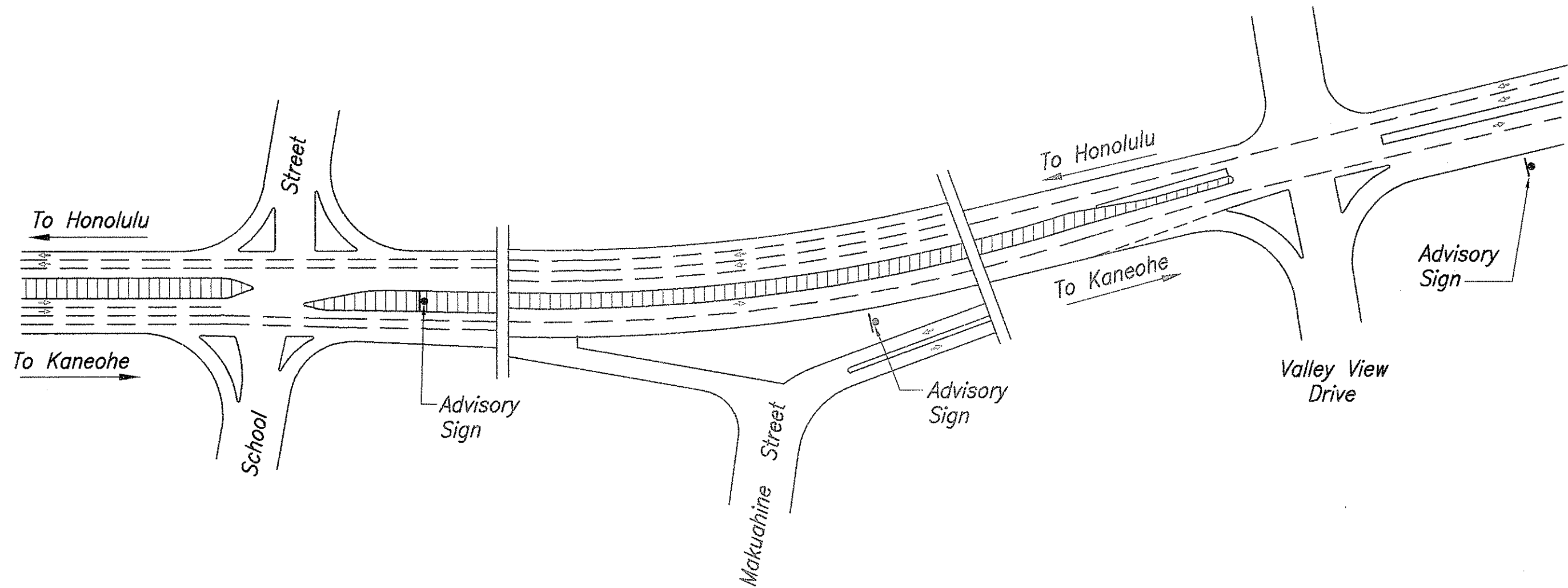
LOCATION OF ADVISORY SIGNS (HONOLULU SIDE) SCALE: NOT TO SCALE
