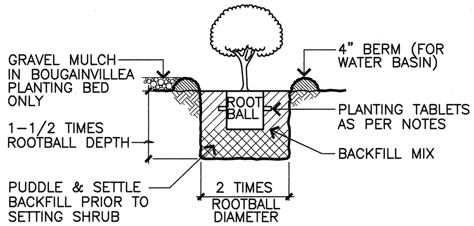
2 SHRUB PLANTING DETAIL NOT TO SCALE
