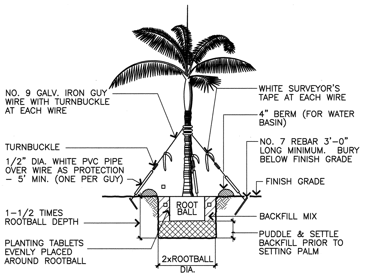
1 RELOCATED PALM PLANTING DETAIL NOT TO SCALE
