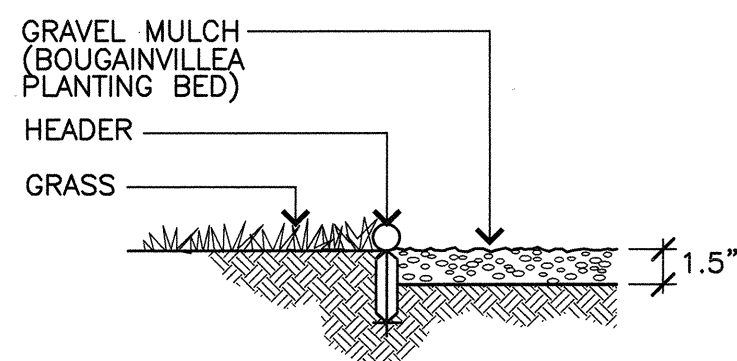
3 PLASTIC HEADER DETAIL NOT TO SCALE
