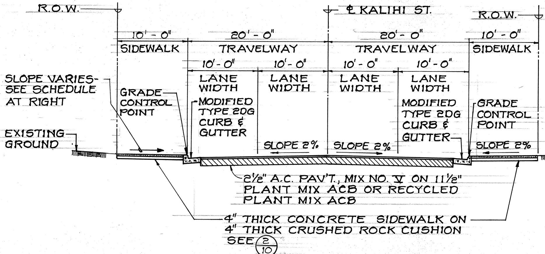
1 TYPICAL ROAD SECTION SCALE: 1/8" = 1'-0"
