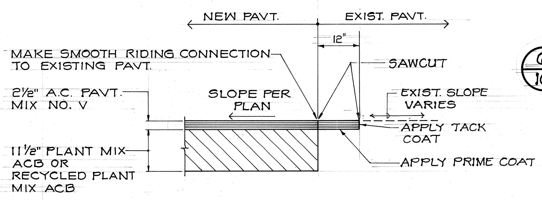
5 PAVEMENT CONNECTION DETAIL NOT TO SCALE
