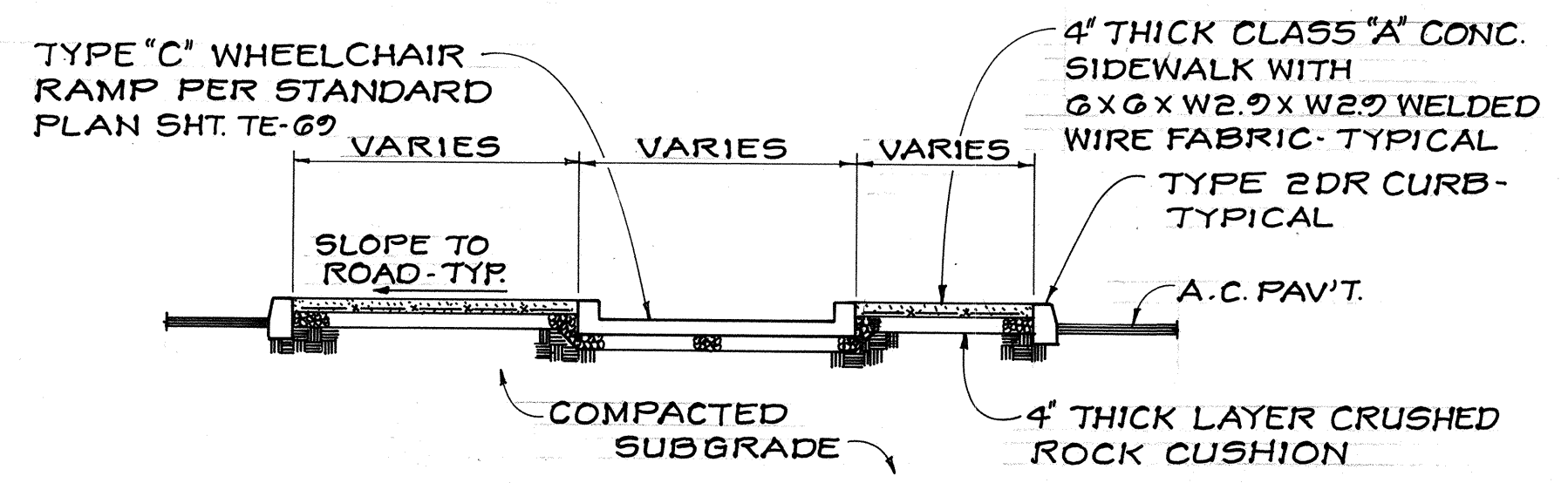
ISLAND TYPICAL SECTION NOT TO SCALE
