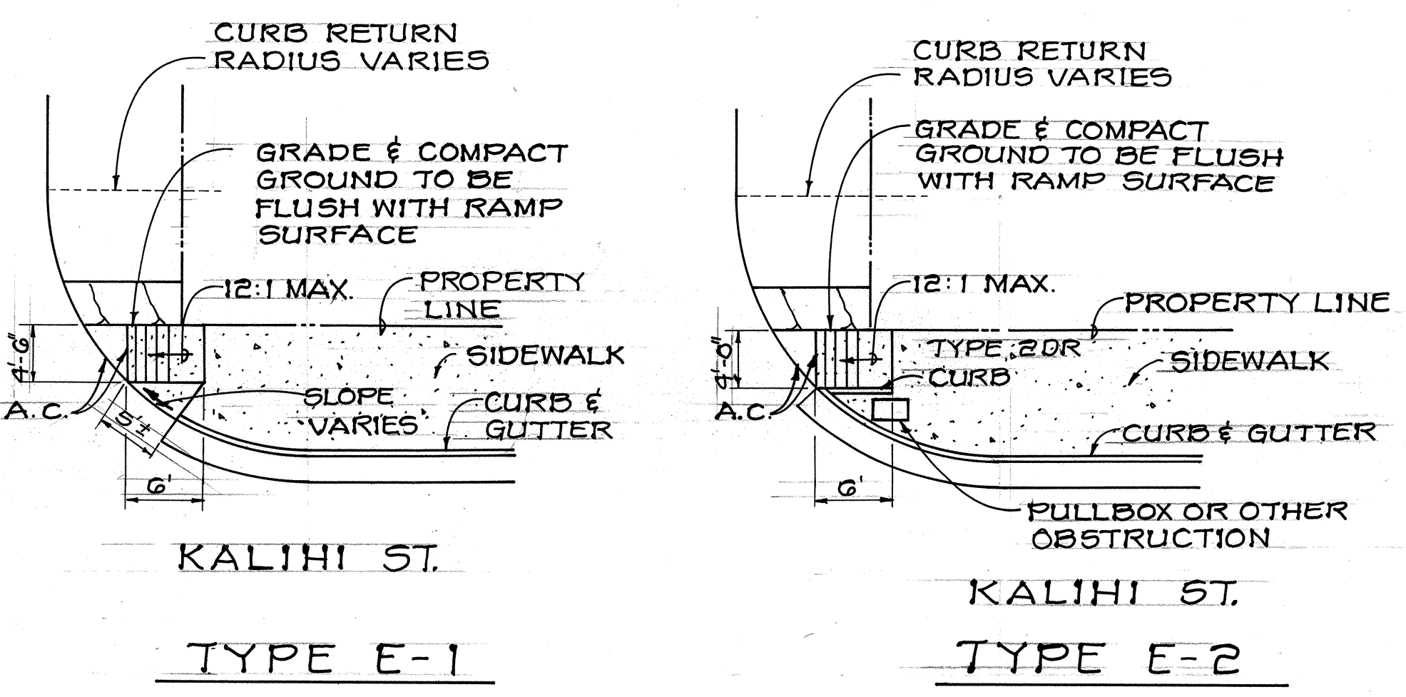
3 MODIFIED TYPE "E" WHEELCHAIR RAMP DETAILS NOT TO SCALE
