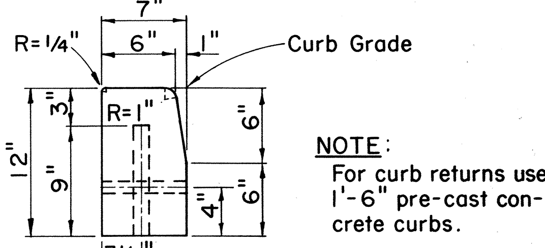
SECTION C-C CURB, TYPE 3D PRE-CAST CONC. CURB Scale: 1 1/2" = 1'-0"
