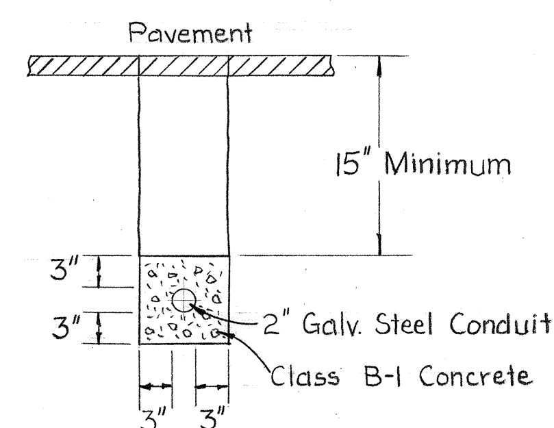
TYPICAL SECTION - ENCASED DUCT NOT TO SCALE
