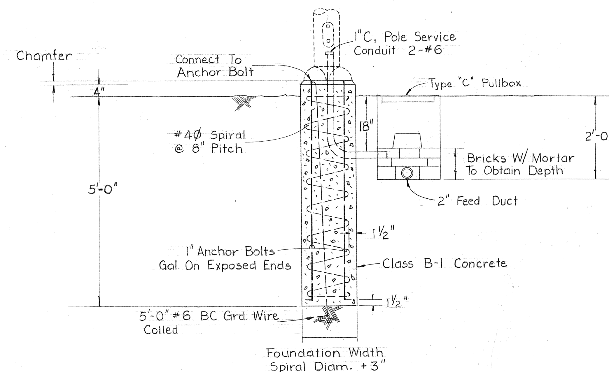
TYPICAL DETAIL - LIGHT STANDARD FOUNDATION NOT TO SCALE
