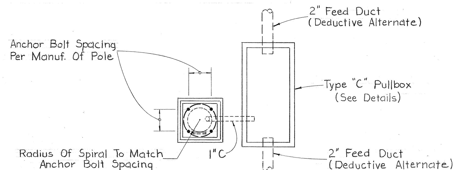
PLAN VIEW - LIGHT STANDARD FOUNDATION NOT TO SCALE
