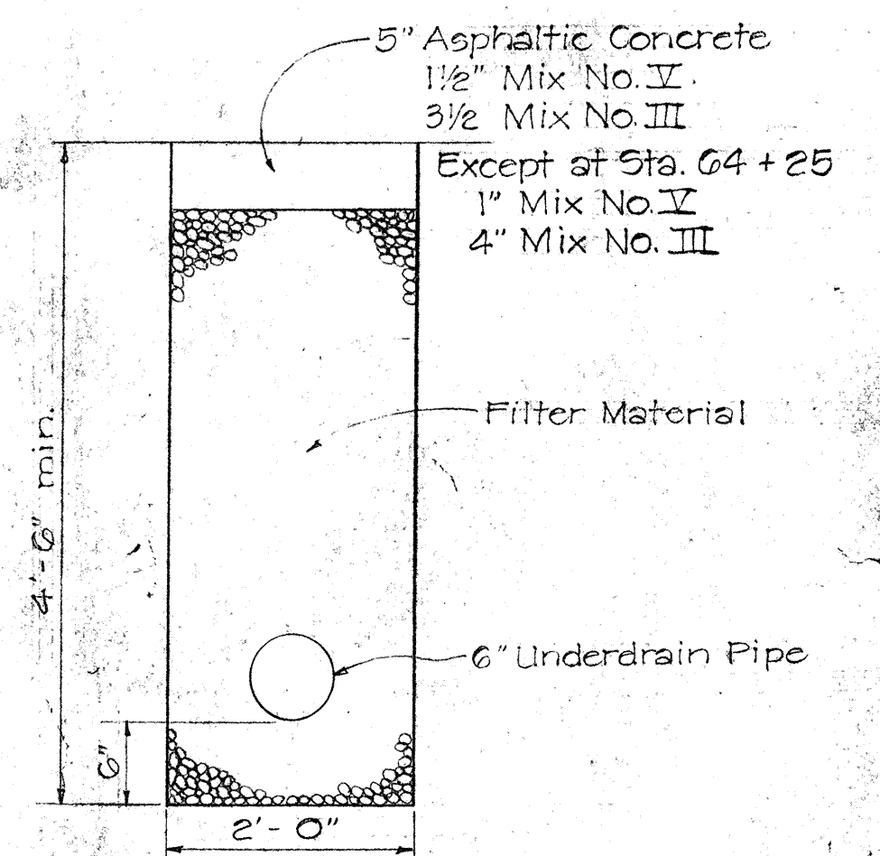
UNDERDRAIN DETAIL
