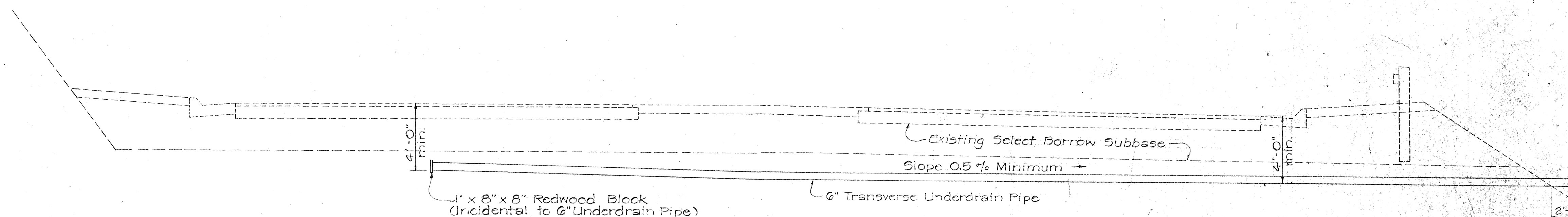
TYPICAL SECTIONS FOR 6" UNDERDRAIN PIPES
