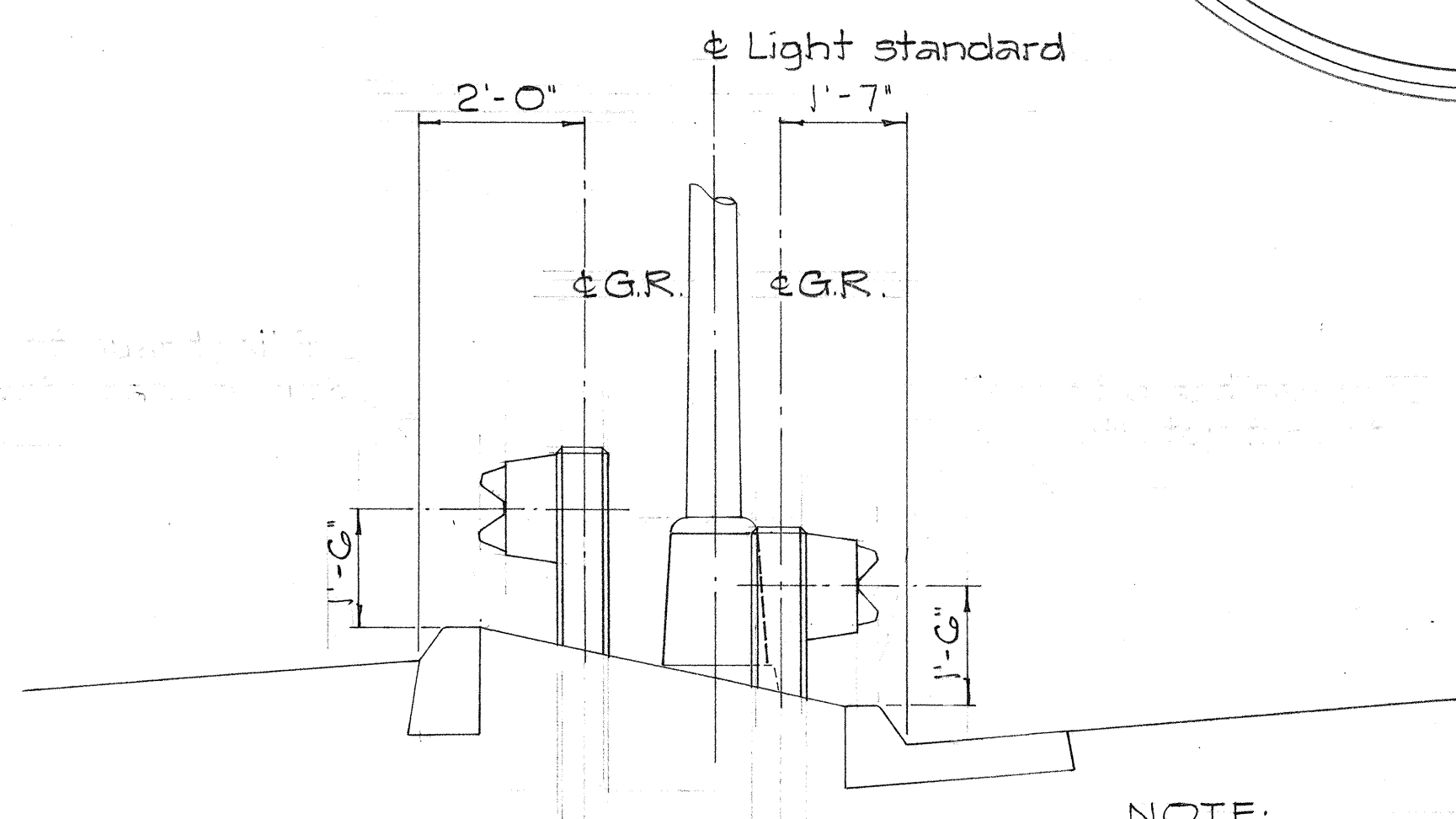
GUARD RAIL DETAIL AT LIGHT STANDARDS #3, #4, #5, #6, #8
