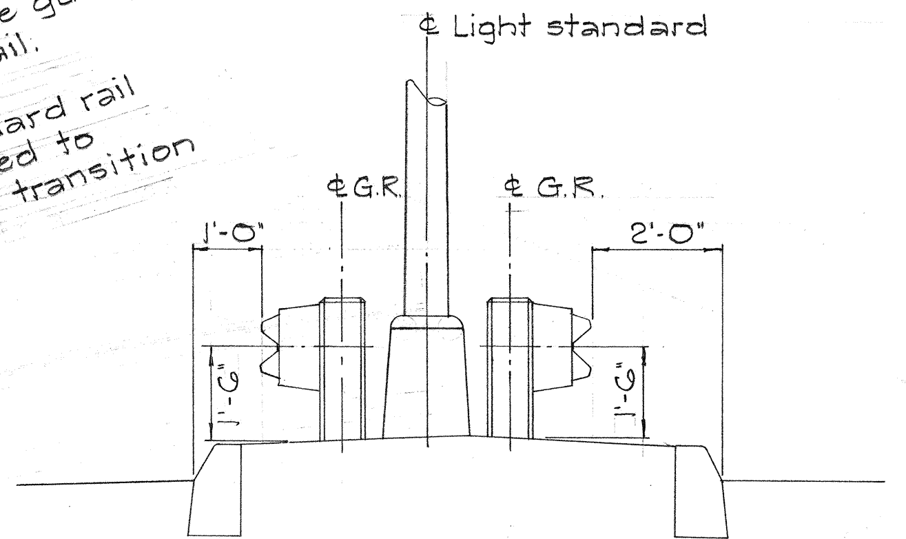
GUARD RAIL DETAIL AT LIGHT STANDARD #7
