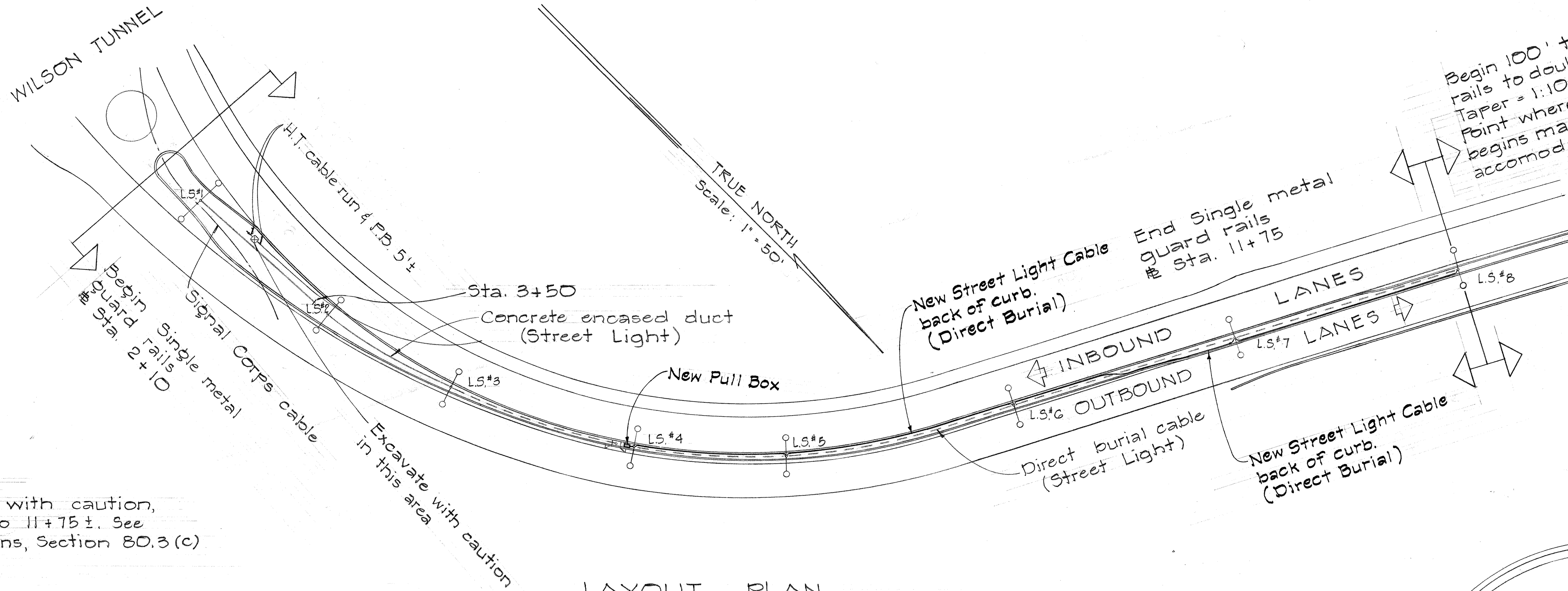
LAYOUT PLAN
