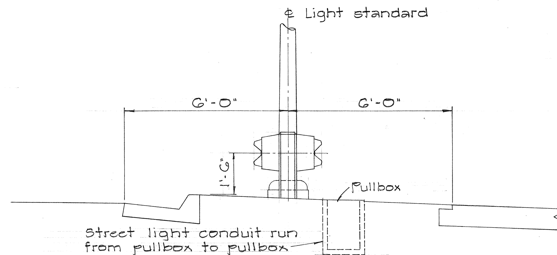
TYPICAL GUARD RAIL DETAIL, MEDIAN CURBED ON ONE SIDE ONLY
