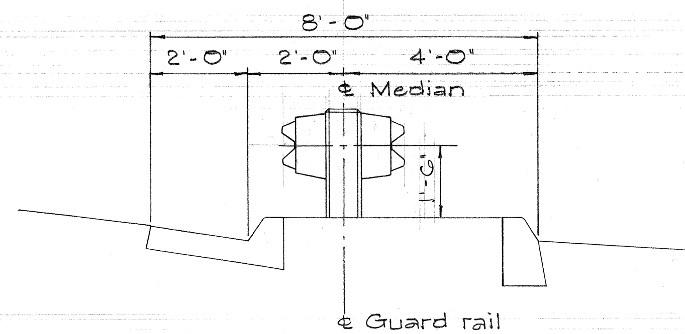
TYPICAL DETAIL, MEDIAN WITH GUTTER
