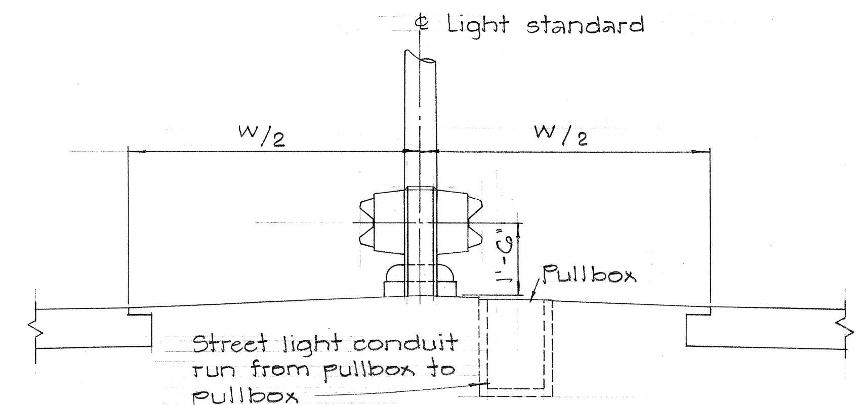
TYPICAL GUARD RAIL DETAIL AT UNCURBED MEDIAN
