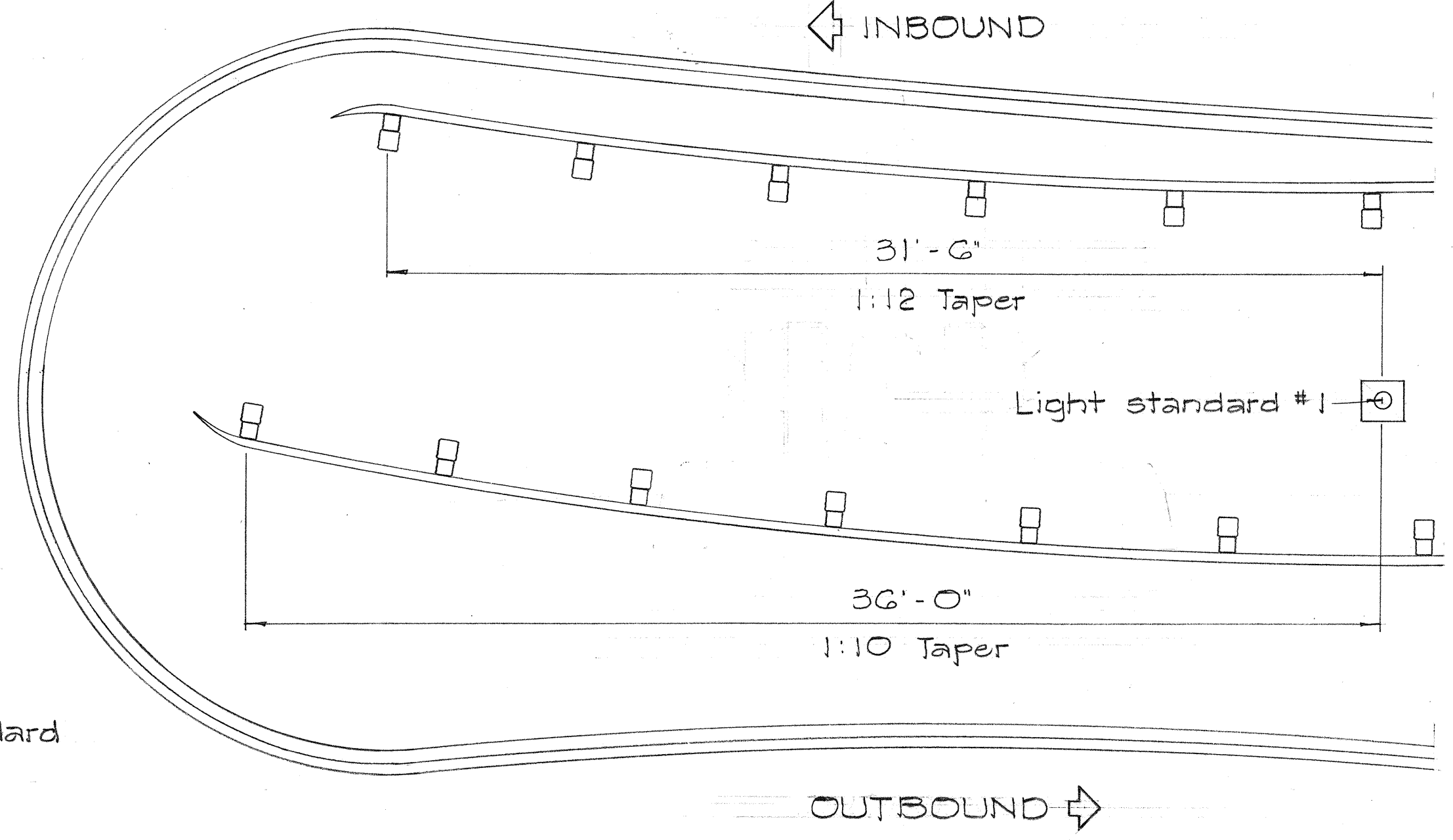
DETAIL OF GUARD RAIL TAPER
