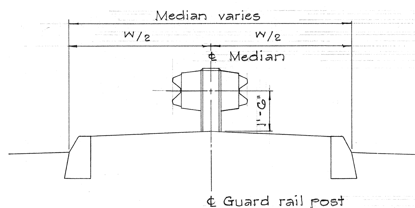
TYPICAL DETAIL, MEDIAN WITHOUT GUTTER
