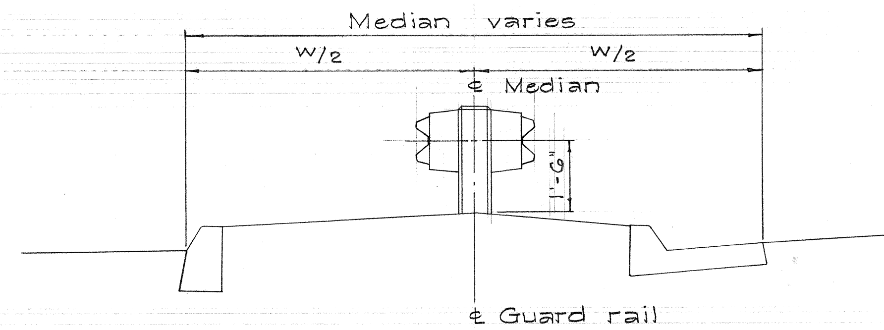
TYPICAL DETAIL, MEDIAN WITH GUTTER
