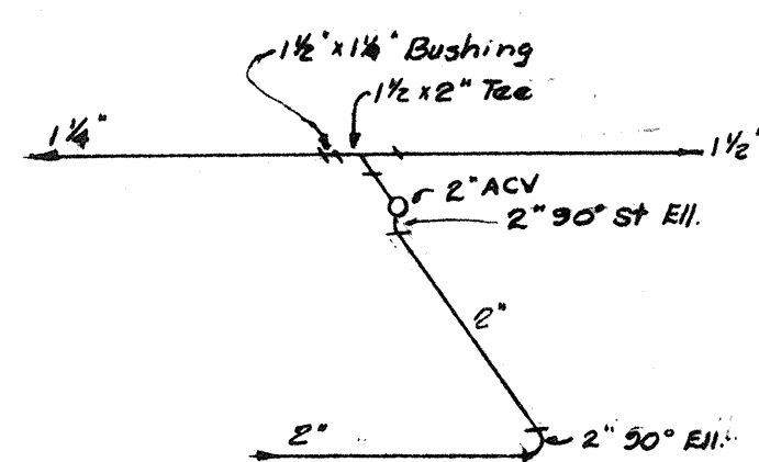
DETAIL 5-B
