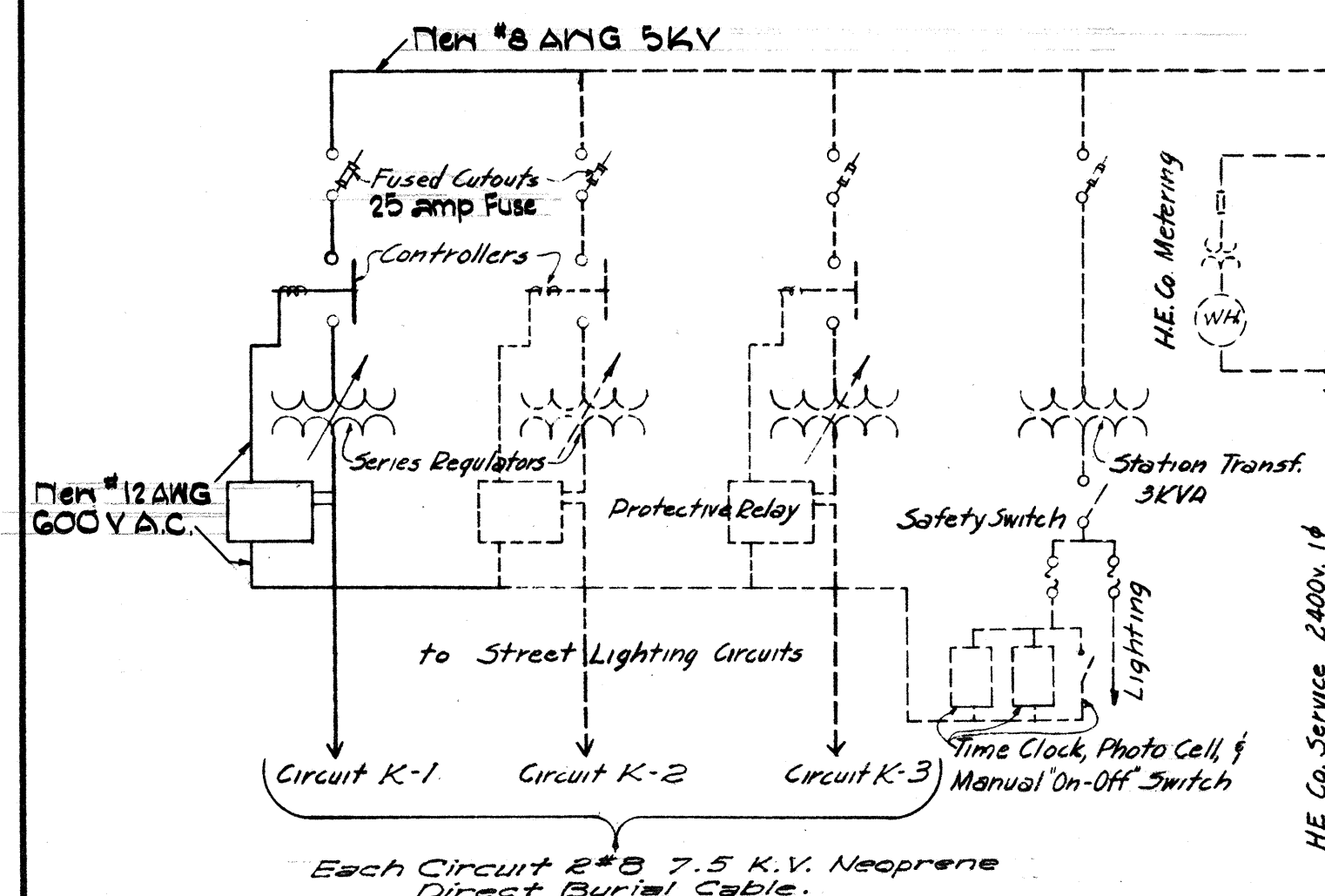
WIRING DIAGRAM SUB-STATION #2 No Scale
