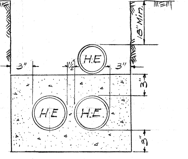
SECTION "C-C" 2-HAW. ELEC. 4" TRANSITE KORDUCT 1-HAW. ELEC. 3" TRANSITE DUCT
