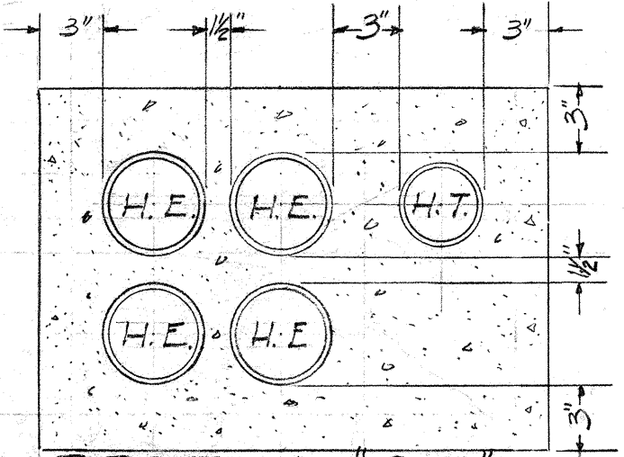
SECTION "G-G" 4-HAW. ELEC. 4" TRANSITE DUCT 1-HAW. TEL. 3/4" TRANSITE KORDUCT
