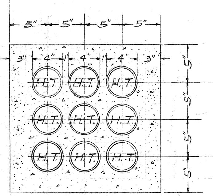
SECTION "X-X" 3-4" HAW. TEL. 3/4" TRANSITE KORDUCT
