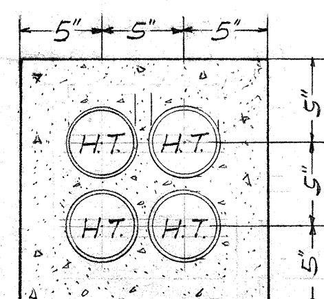
SECTION "B-B" 4-HAW TEL 3 1/2" TRANSITE KORDUCT
