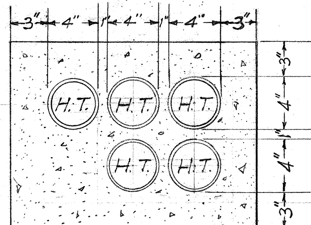
SECTION "E-E" 5-HAW TEL 3 1/2" TRANSITE KORDUCT
