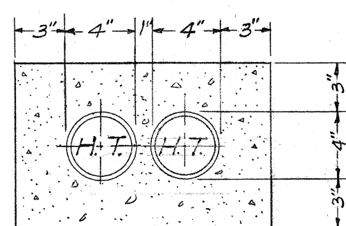
SECTION "A-A" 2-HAW TEL 3 1/2" TRANSITE KORDUCT
