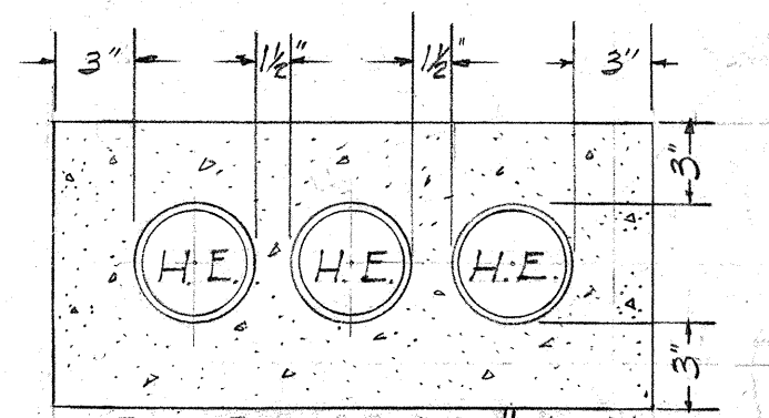
SECTION "J-J" 3-4" TRANSITE DUCT
