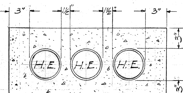
SECTION "D-D" 3-HAW TEL 4" TRANSITE DUCT
