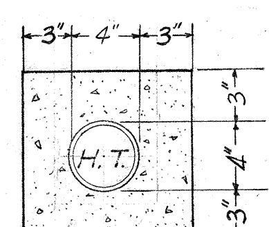
SECTION "F-F" 1-HAW TEL 3 1/2" TRANSITE KORDUCT
