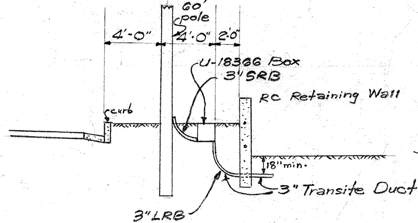
DETAIL OF UNDERGROUND SERVICE TO YMCA Not to scale
