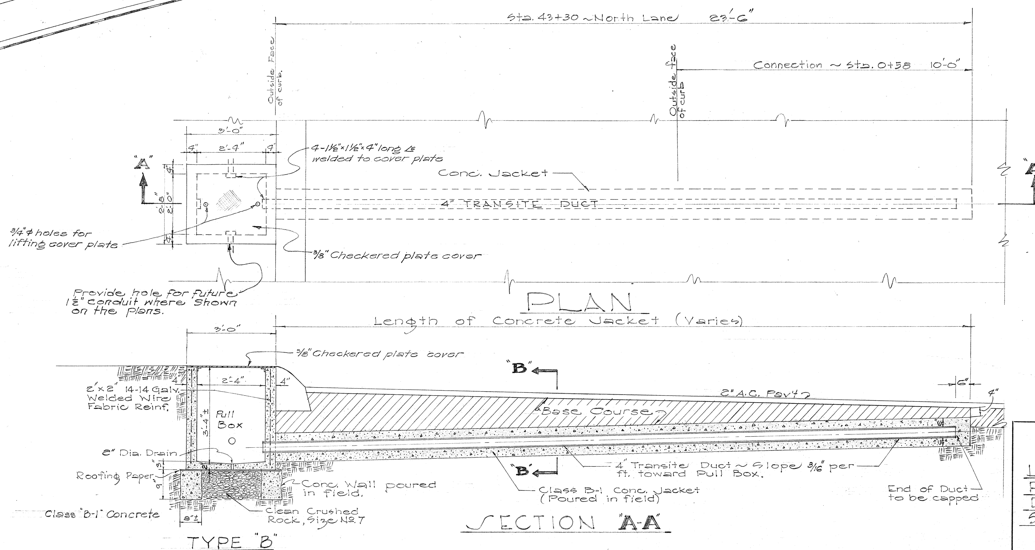
DETAIL OF PULL BOX & TRANSITE DUCT Scale: 1/2" = 1'-0"
