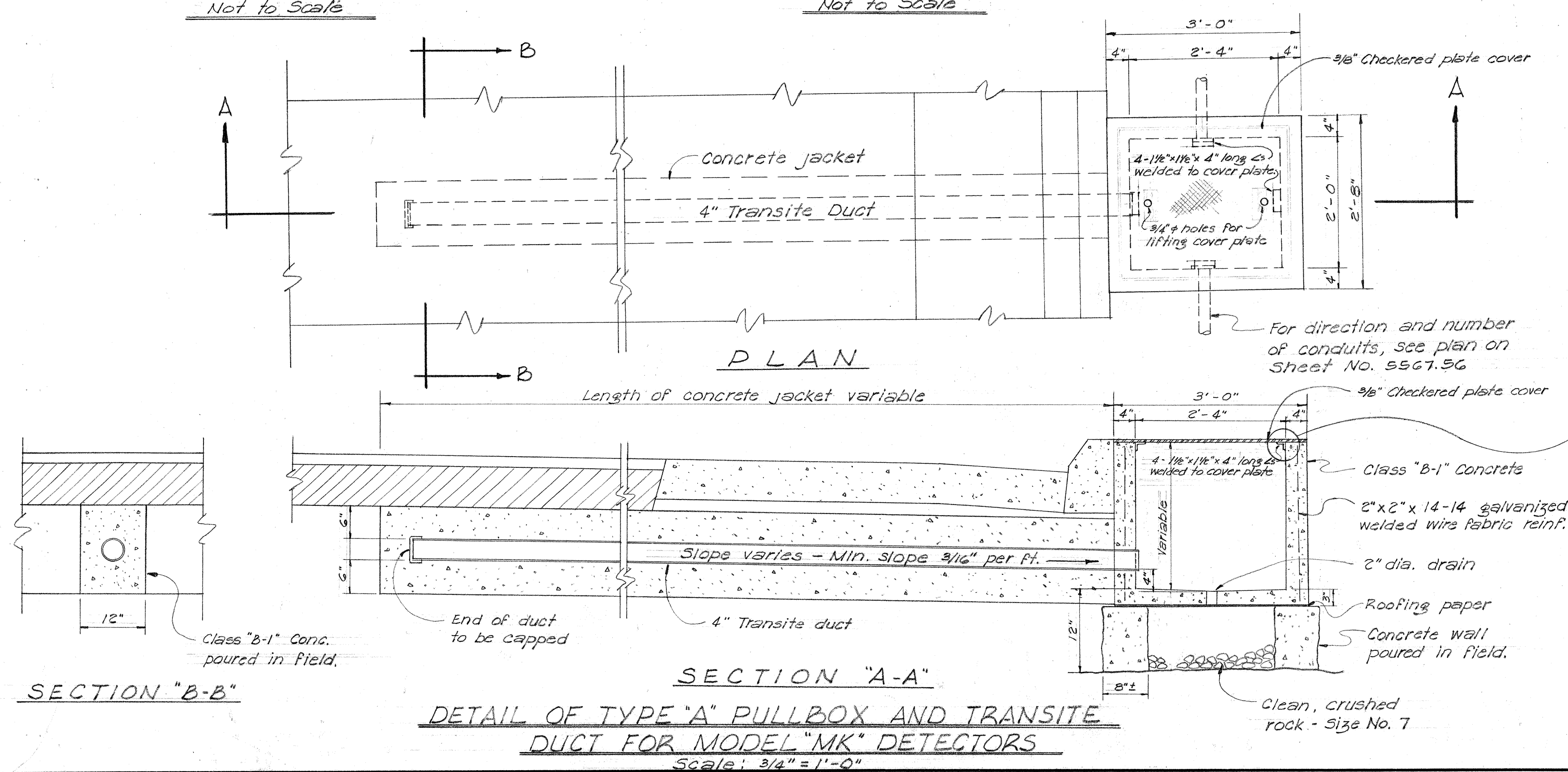
SECTION "A-A"
