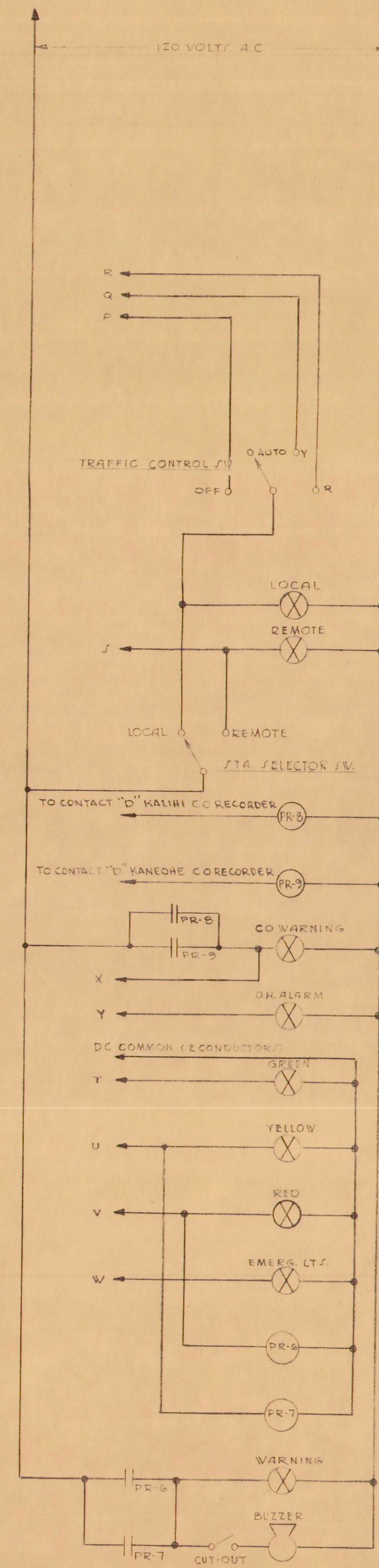
TRAFFIC SIGNAL SYSTEM SECTION OF MAIN CONTROL SWITCHBOARD
