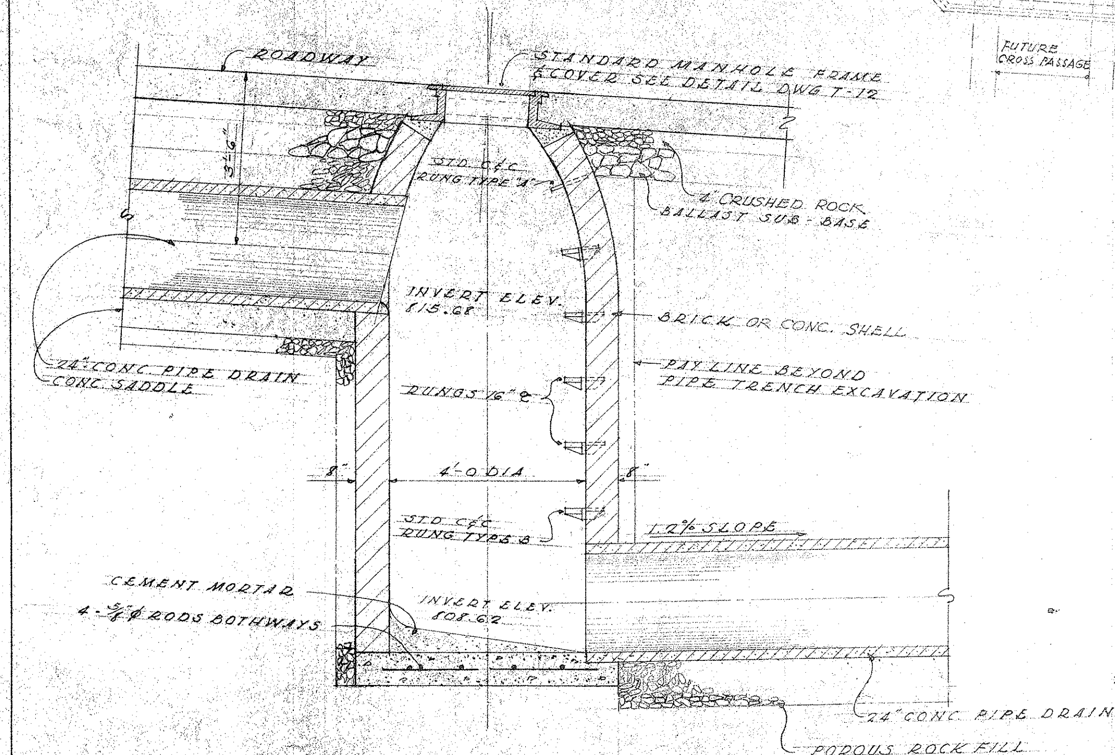
DROP MANHOLE DETAIL SCALE: 1/2\"/>
