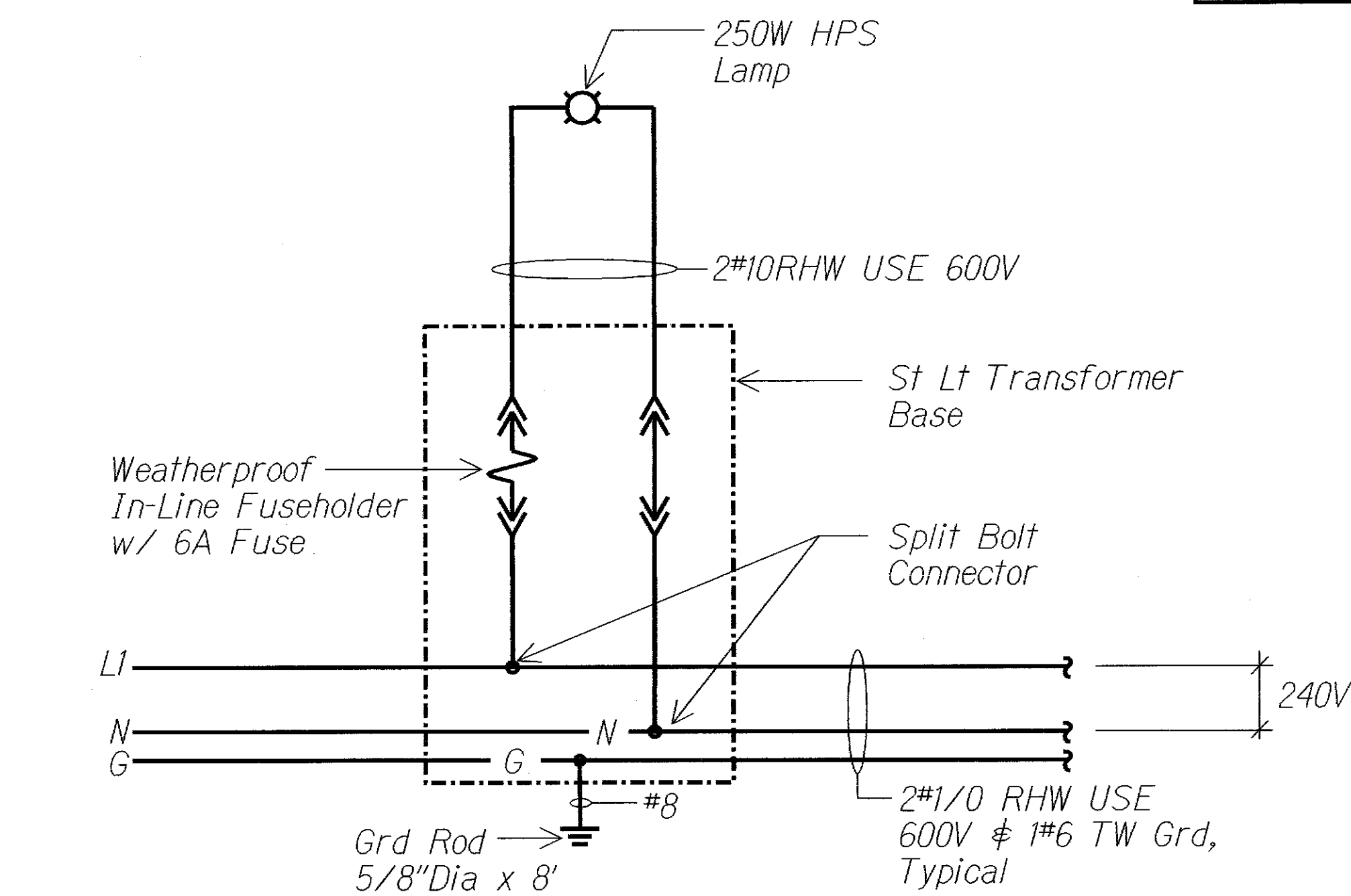
TYPICAL STREET LIGHT WIRING DIAGRAM
