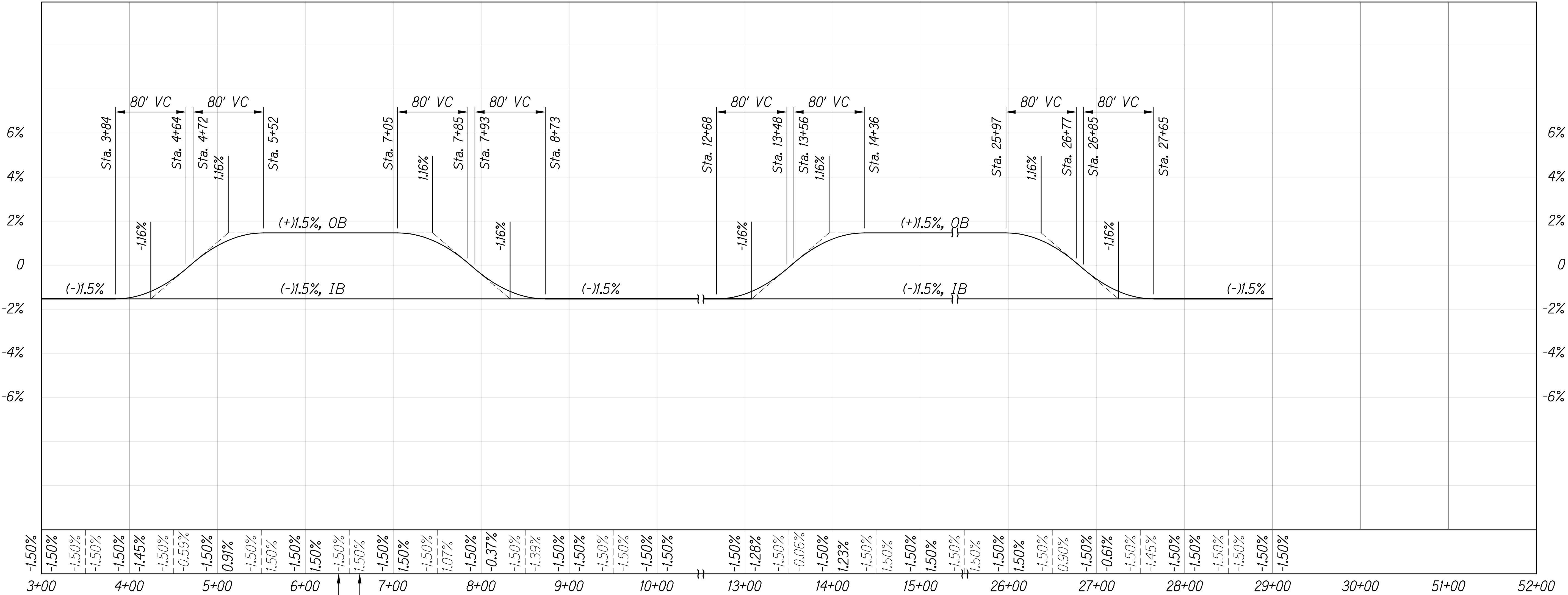
CURVE #9 PC @ Sta. 4+97.80 to PT @ Sta. 7+59.60
