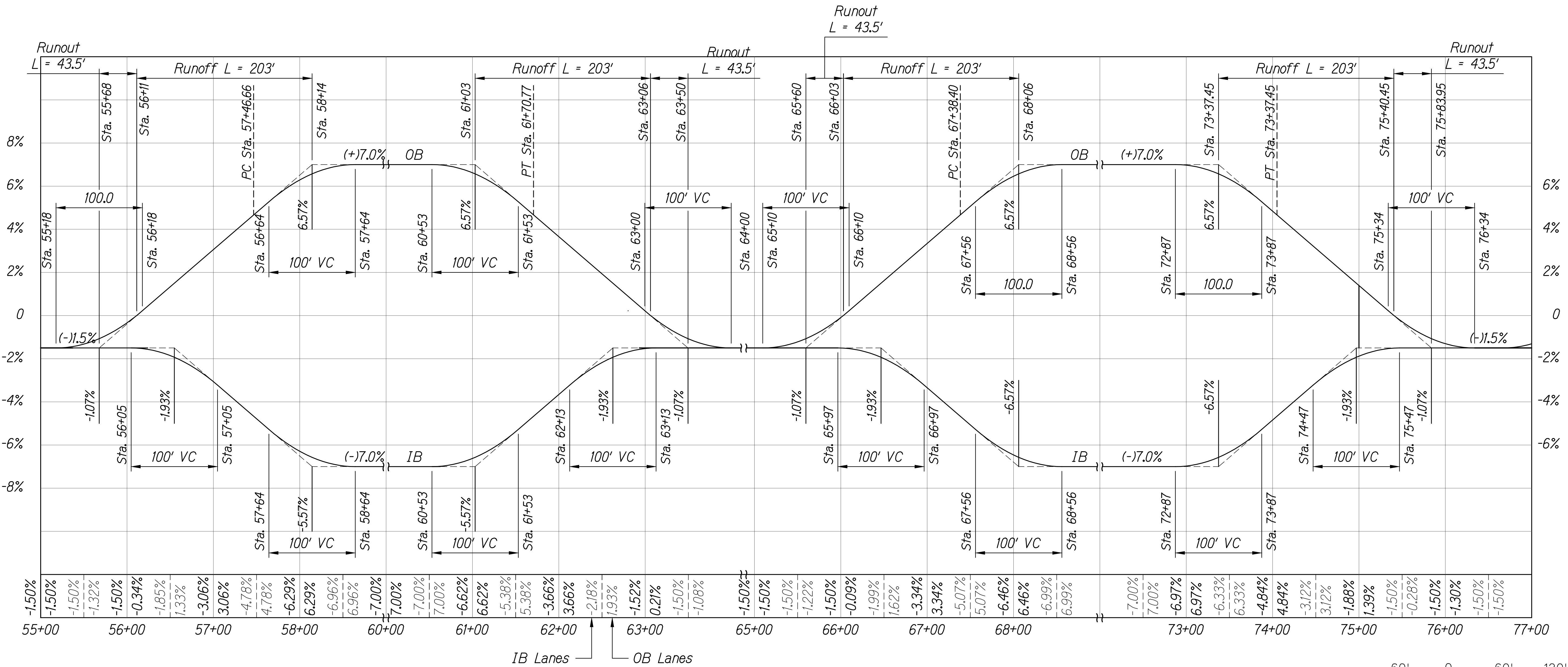
CURVE #3 PC @ Sta. 57+46.66 to PT @ Sta. 61+70.77
