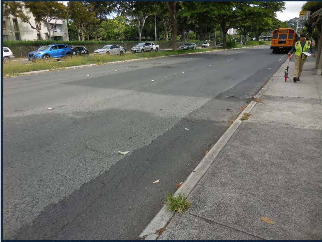
Photo No. 1: Heavy rutting under bus wheel path.
